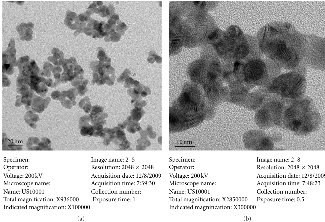
FIGURE 1: TEM images of Ag-NPs used in the experiments.
