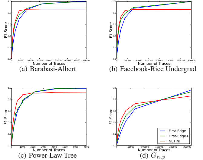
Figure 2: F1 score of the First-Edge, First-Edge+, and NETINF algorithms applied to different real and synthetic networks against a varying number of traces. (best viewed in color)
