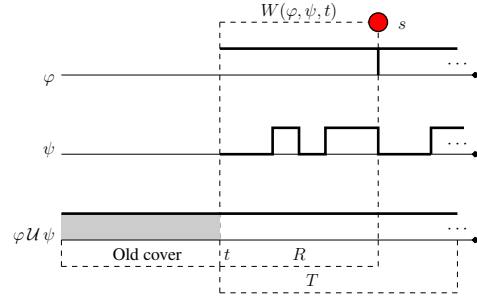
Fig. 3. (a) Algorithm to find a correct instance of \xi_{\varphi \mathcal{U} \psi} over T relative to signal w ; (b) Example of R and s computation for \varphi \mathcal{U} \psi .
