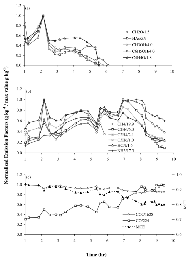
Figure 1. The trace gases detected by OP-FTIR in the smoke from the Northwest Territories Organic Soil 1 fire are shown as normalized IEF versus hours since ignition. (Specifically, each IEF is divided by the maximum IEF, which is shown in the legend.) The emissions are grouped according to their formation process: (a) the products of low-temperature pyrolysis of fresh biomass, which creates “low-temperature char,” (b) the products of high-temperature pyrolysis of low-temperature char, and (c) the products of gasification. Part (c) also shows the MCE.
