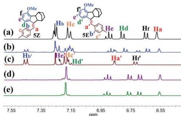
Fig. 2 1 H NMR spectra of 5Z (a) in CDCl 3 sealed with K 2 CO 3 , (b) in newly opened CDCl 3 (which contains a tiny amount of acid), (c) with addition of 0.5 eq. of TFA to CDCl 3 , (d) in DMSO- d 6 measured soon after preparing the solution, and (e) in DMSO- d 6 after heating at 130 °C for 24 h. All measurements were performed at room temperature.
