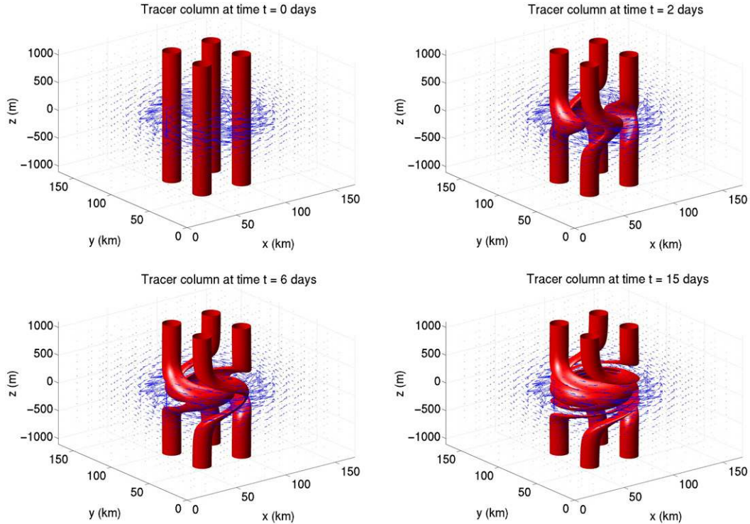
FIG. 8. 3D view of the tracer columns deformation at time = 0, 2, 6, and 15 days in the tangent linear model. The blue arrows are the velocity vectors. An intense differential winding of the tracer tubes by the vortex velocity field yields to the formation of vertical variability.
