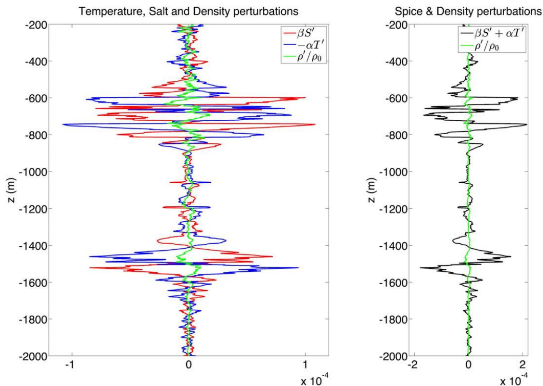
FIG. 3. (a) Contribution of temperature (blue) and salinity (red) in the density perturbation (green) near a meddy rotation axis. (b) Associated spice (black) and density (green) perturbation. Layering in tracer fields is observed above and below the meddy. Salinity effects on density compensate temperatures at 90% in the filtered density field. T , S , and the density have been filtered with a high-pass filter ( <200 m).
