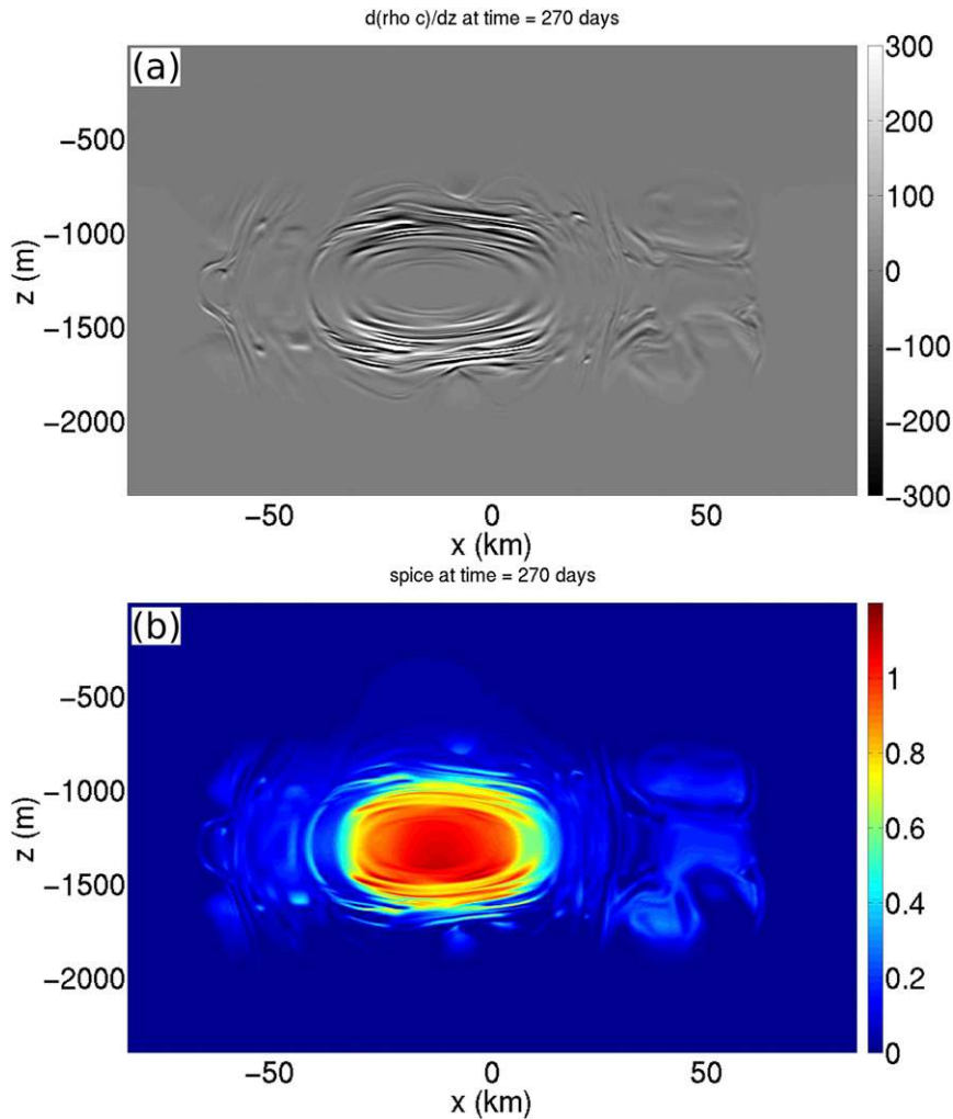
FIG. 4. (a) Vertical section of acoustic reflectivity in the central part of the vortex after 270 days of PE model integration. (b) As in (a), but for the spice variable. Layering is obvious both in acoustic reflectivity and spice.
