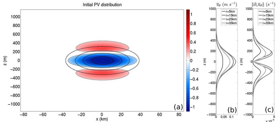
FIG. 2. (a) PVA distribution of the meddy-like vortex lens (nondimensional). The thick gray lines represent the -0.2 and 0.1 PVA contours, while the black dotted lines represent the associated streamfunction contours. (b) Vertical profiles of the azimuthal velocity at 5, 15, 25, and 35 km from the vortex rotation axis. (c) As in (b), but for the absolute value of the vertical shear of the azimuthal velocity.
