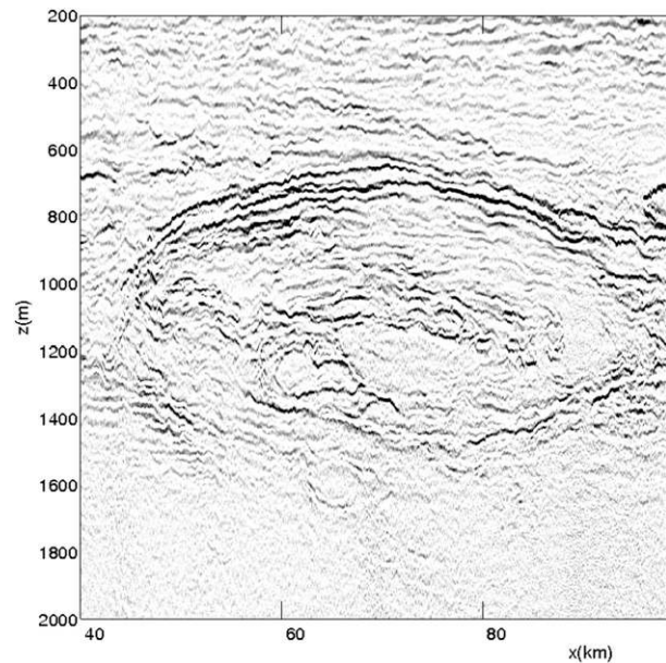
FIG. 1. Seismic reflectivity of the Meddy GO, adapted from Hua et al. (2013). The reflectors are doming all around the meddy, similar to Biescas et al. (2014).
