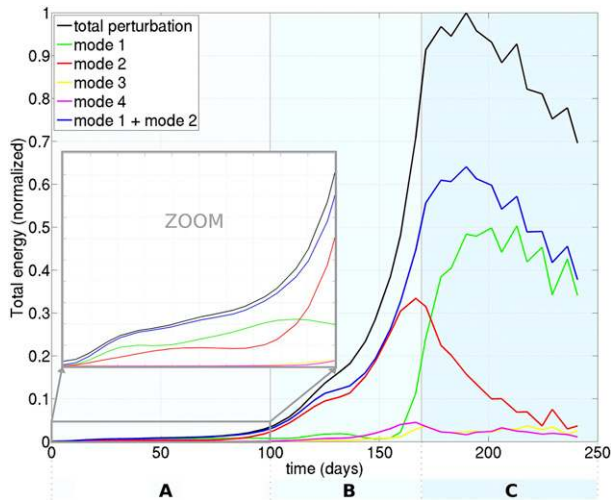
FIG. 13. Time evolution of the perturbation energy in the non-linear QG simulations. The black line is the total perturbation energy while the green, red, yellow, purple, and blue lines are, respectively, the energy of azimuthal modes 1, 2, 3, and 4 and the sum of modes 1 and 2. Most of the total perturbation energy is contained by the first two modes.
