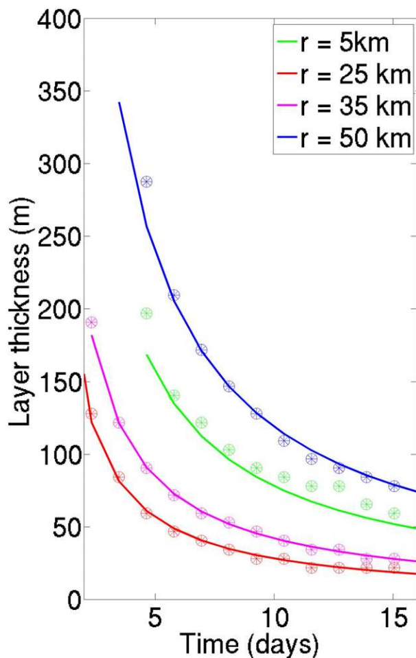
FIG. 10. Time evolution of the layer thicknesses in the isolated tracer column experiments for four different initial positions of the column. The circled asterisks represent the thickness measured from the model outputs, while the plain lines represent the theoretical thickness inferred from Eq. (14). The simple linear scaling is a good estimation of the thinning of the layers.
