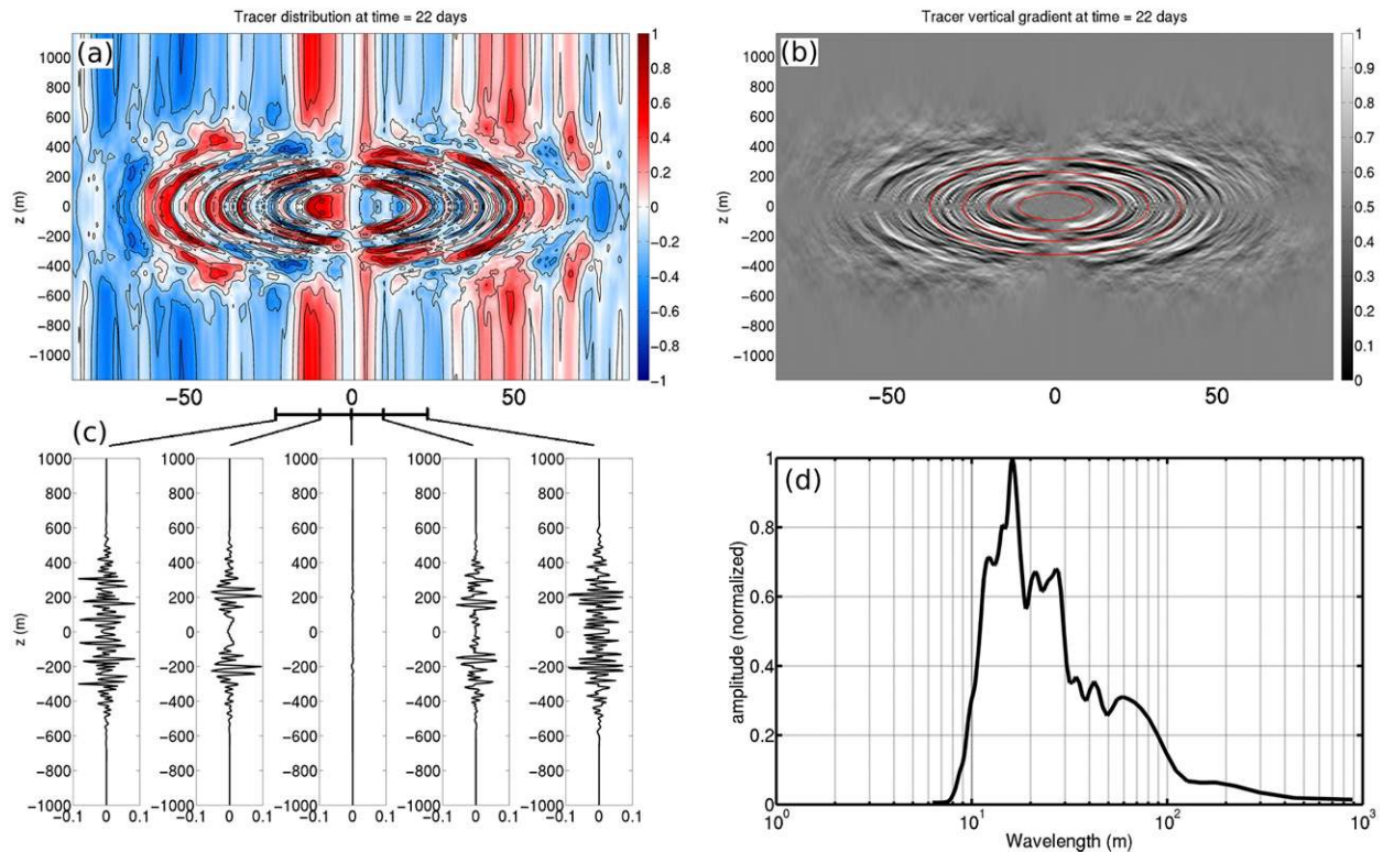
FIG. 7. As in Fig. 6, but after 22 days of model integration. Layering has increased with time, while the vertical length scale has decreased.
