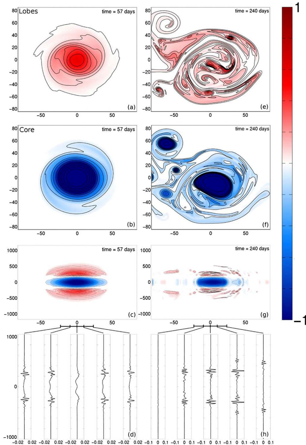
FIG. 12. Snapshots from the nonlinear QG simulations after (left) 57 and (right) 240 days of model run. (a),(e) QGPV horizontal section in the eddy lobes. (b),(f) QGPV horizontal section in the eddy core. (c),(g) QGPV vertical section. (d),(h) Vertical profiles of high-pass filtered QGPV perturbation at five distinct locations. Layering starts to develop during the linear stage of destabilization. It is greatly enhanced once the vortex lobes have reached a nearly turbulent state.
