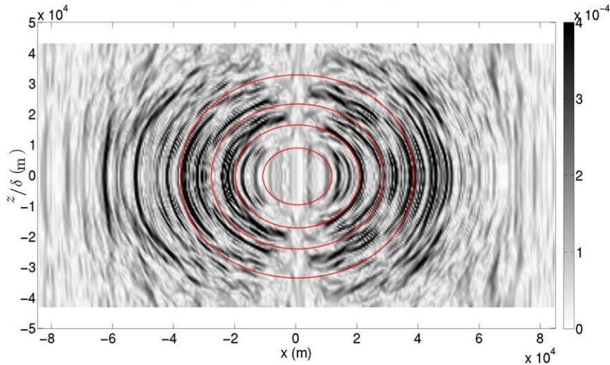
FIG. 11. Radial tracer gradient in stretched coordinates after 22 days of integration of the tracer model. The z axis was stretched by the vortex aspect ratio. Layers are concentric rather than properly vertically stacked.
