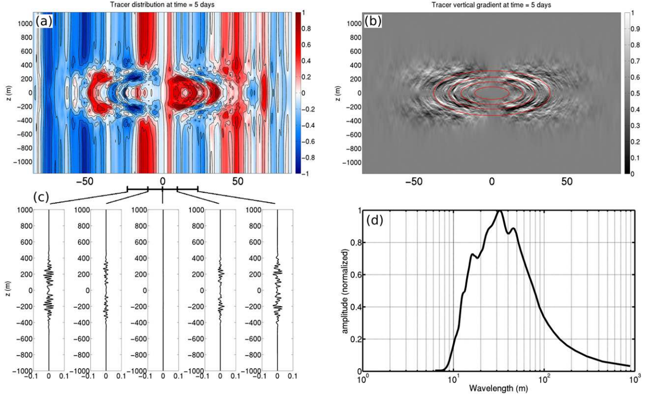
FIG. 6. Tracer properties after 5 days of model integration: (a) vertical section of the tracer concentration (normalized); (b) vertical section of the tracer's vertical gradient (normalized); (c) vertical profiles of tracer anomaly; and (d) spectral distribution of the tracer vertical anomaly. The baroclinization of the tracer field is evident from the first days of model integration.
