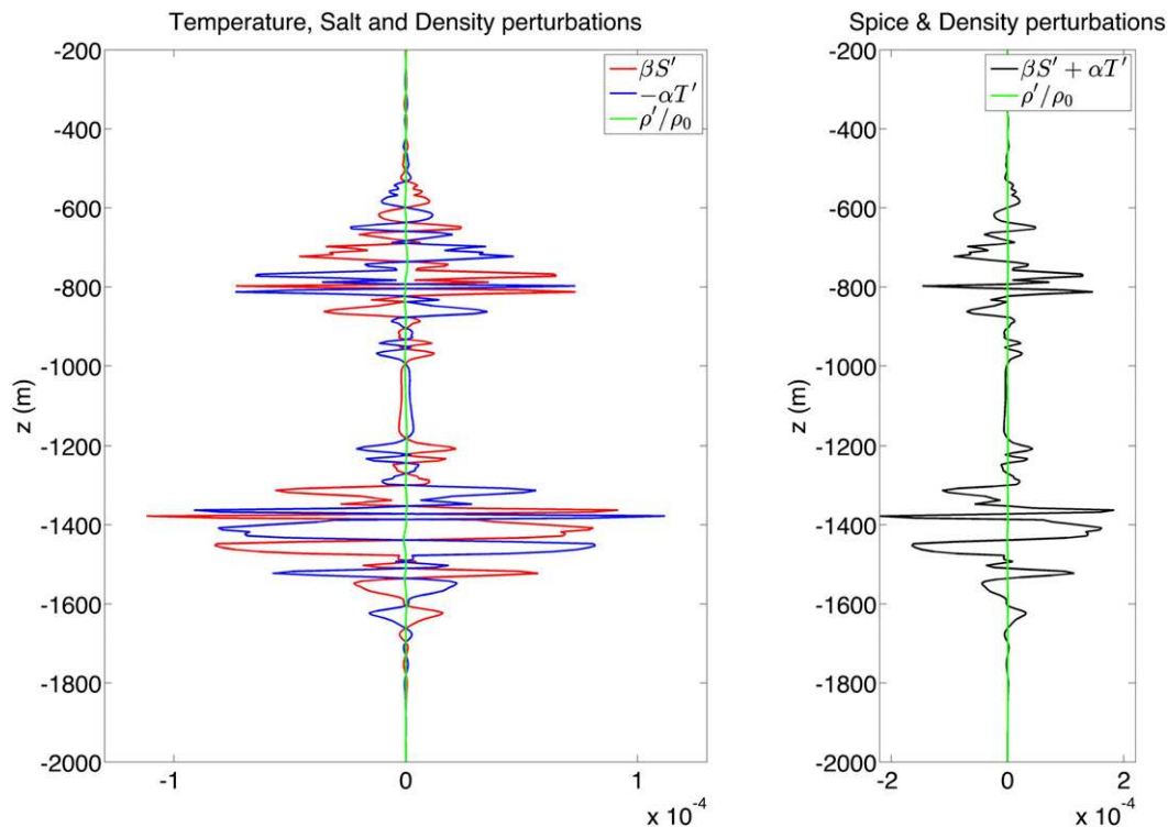
FIG. 5. As in Fig. 3, but for the modeled meddy. Strong anomalies in temperature and salinity result in strong spice anomalies while the density is almost unaffected.
