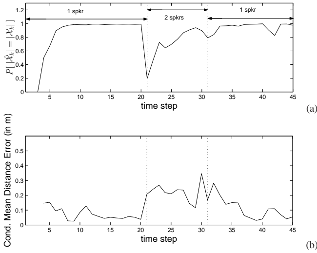
Fig. 9. Average location tracking performance of the multi-speaker RFS SMC filter in Example 1.
