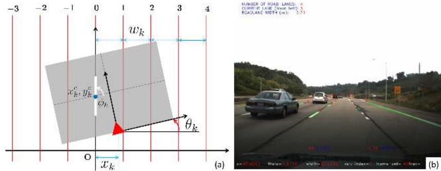
Figure 1: (a) A model of a road-plane. (b) An example output of lateral localization. At the top-left, the information about ego-vehicle’s lateral location is displayed. The green pixel blobs are the detected lane-marrings. The red numbers on the green pixel blobs represent lane-marking group identifiers.
