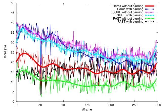
Figure 7: Recall values obtained in the Posters sequence.
