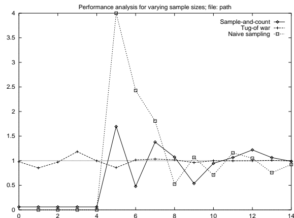
Figure 1: A pathological example, in which the three algorithms are run on a data set with 40,000 values occurring exactly once, and one value occurring 800 times. The x -axis depicts the base two logarithm of the sample size. The y -axis depicts the normalized value of the estimator, i.e., the ratio of the estimator to the actual self-join size. The horizontal line represents the target normalized value of 1. For each of the 3 algorithms, the normalized value of the estimator is plotted as a function of the sample size used to compute the estimator, for sample sizes 2^i , i = 0, 1, 2, \dots, 14 .
