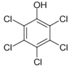
Pentachlorophenol (PCP)
