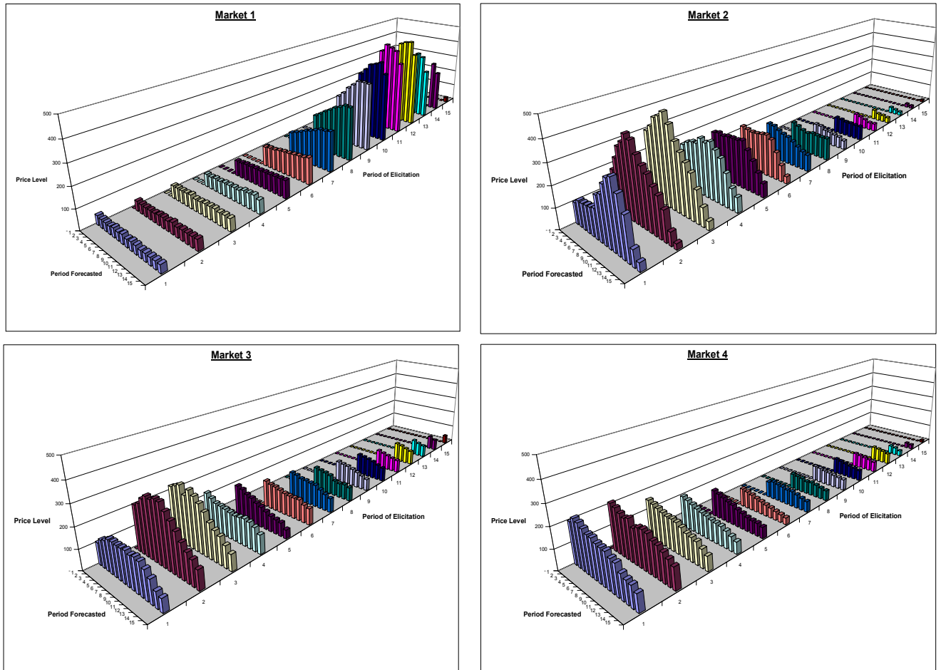
Figure 3: Average prediction for each period in each market, session 2
