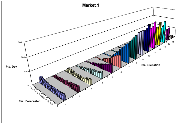
Figure 4: Standard deviation of predictions between subjects in each period for each market, session 2
