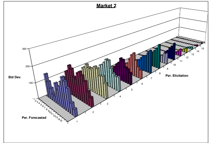
Figure 4: Standard deviation of predictions between subjects in each period for each market, session 2
