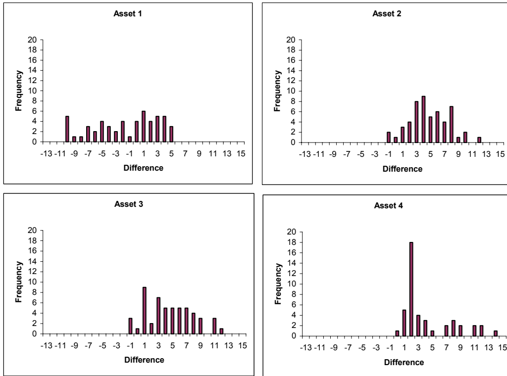
Figure 5. Difference between observed and predicted peak price period, elicitation period 3, all markets and individuals (Positive difference indicates that peak occurred later than predicted)
