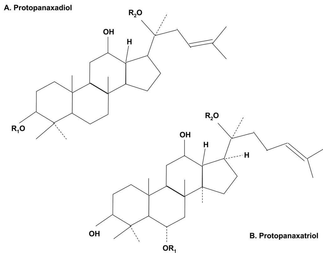
Fig. 1. Structure of ginsenosides (ginseng-specific saponins). A. The ginseng saponins of protopanaxadiol include Ra1, Ra2, Ra3, Rb1, Rb2, Rb3, Rc, Rd, Rg2, Rg3, Rs1, Rs2, et al. B. The ginseng saponins of protopanaxatriol include Re, Rf, Rg1, Rg2, Rh1, et al.
