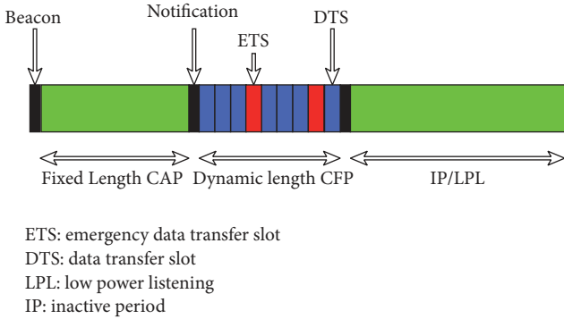
FIGURE 5: Superframe structure of PLA-MAC [21].
