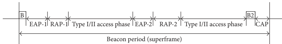
FIGURE 2: IEEE 802.15.6 superframe structure [78].
