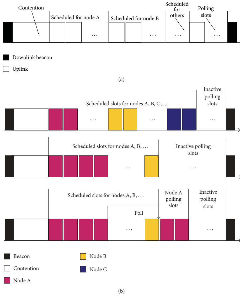
FIGURE 8: (a) Superframe structure of CA-MAC. (b) Dynamic traffic adjustment of contention-free slots in the superframe [22].
