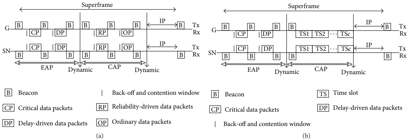
FIGURE 6: Superframe structure for (a) low load and (b) moderate load, high load, and overload [26].
