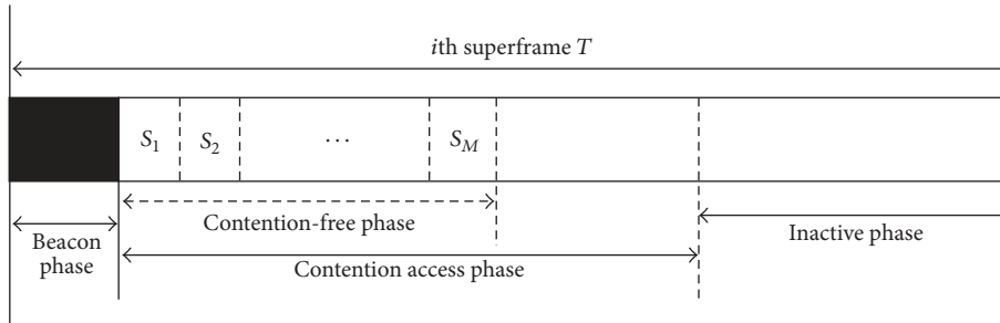
FIGURE 10: Contention over reservation based superframe structure of CoR-MAC [77].
