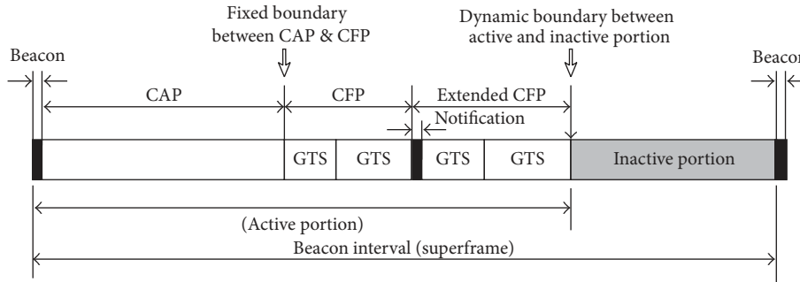
FIGURE 7: The superframe structure of LDTA-MAC [20].
