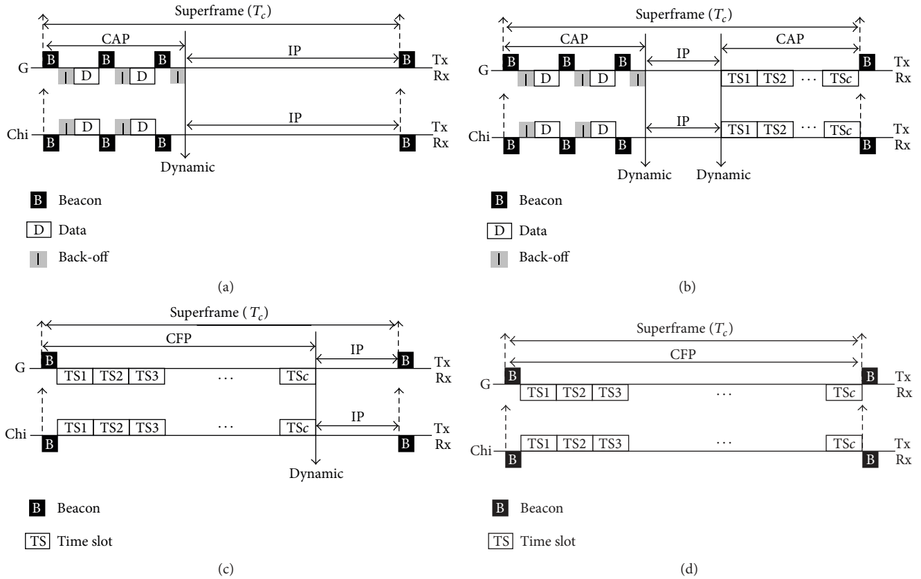
FIGURE 4: Communication from cluster head to gateway (Chi-to-G): (a) low load, (b) moderate load, (c) high load, and (d) overload [3].
