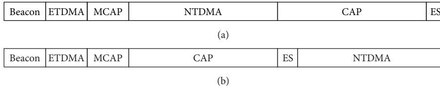
FIGURE 9: Superframe of CAC-MAC [23].
