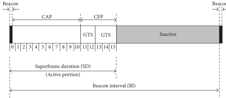
FIGURE 1: General overview of MAC superframe structure of IEEE 802.15.4 beacon-enabled mode [50].
