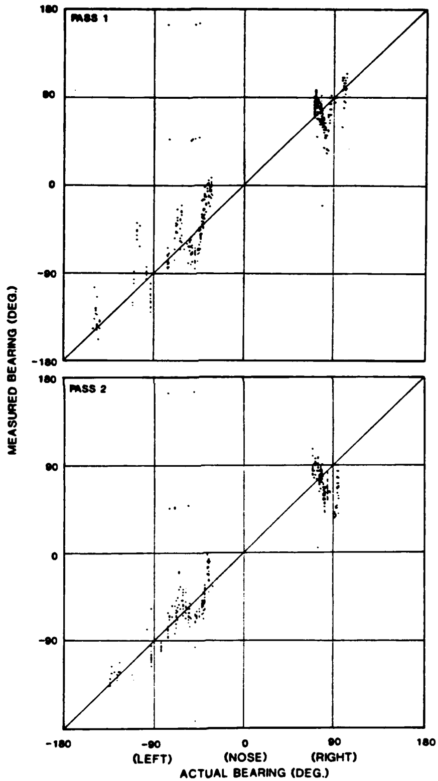
Fig. 4-4. AOA transfer function, two eastbound passes.
