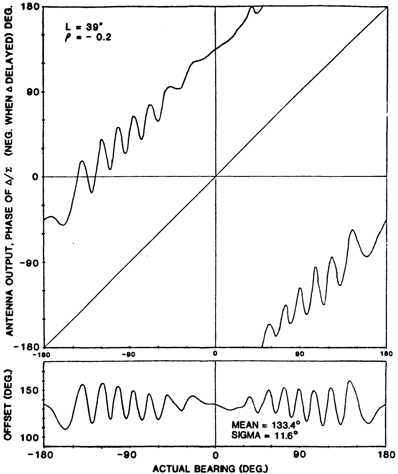
Fig. A-6. Calculated antenna performance with reflector 39 inches away.
