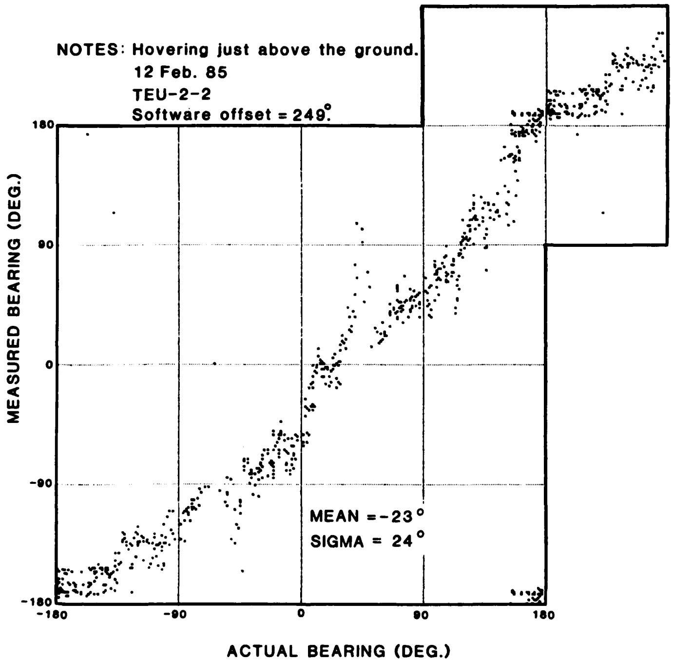
Fig. 4-12. AOA transfer function, top-aft helicopter antenna.
