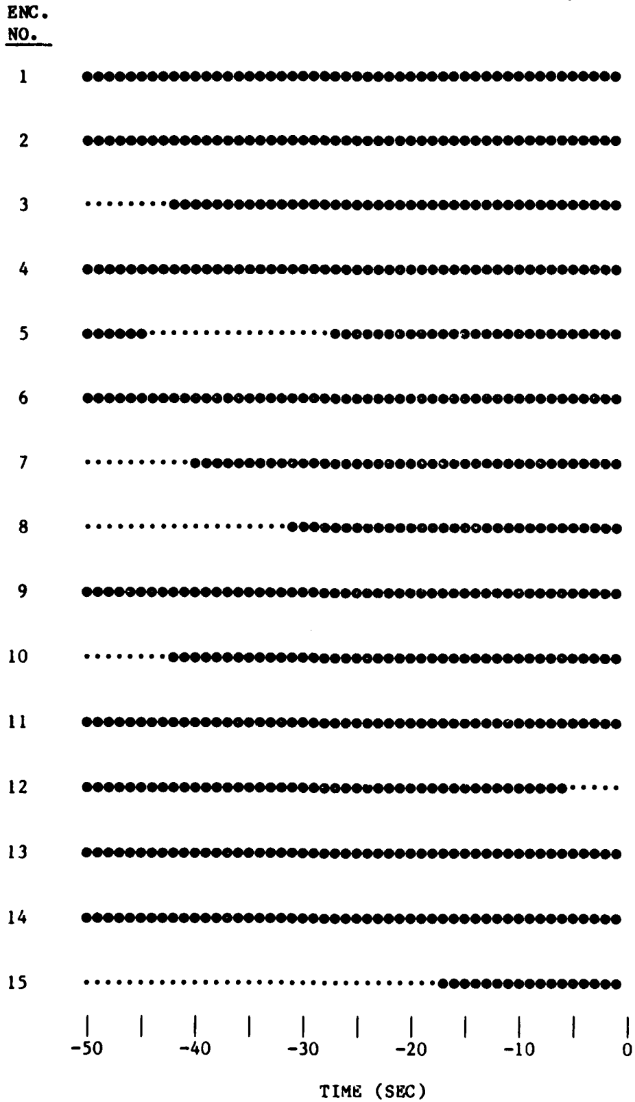
Fig. 3-10. TCAS air-air surveillance during 15 close encounters in New York.
