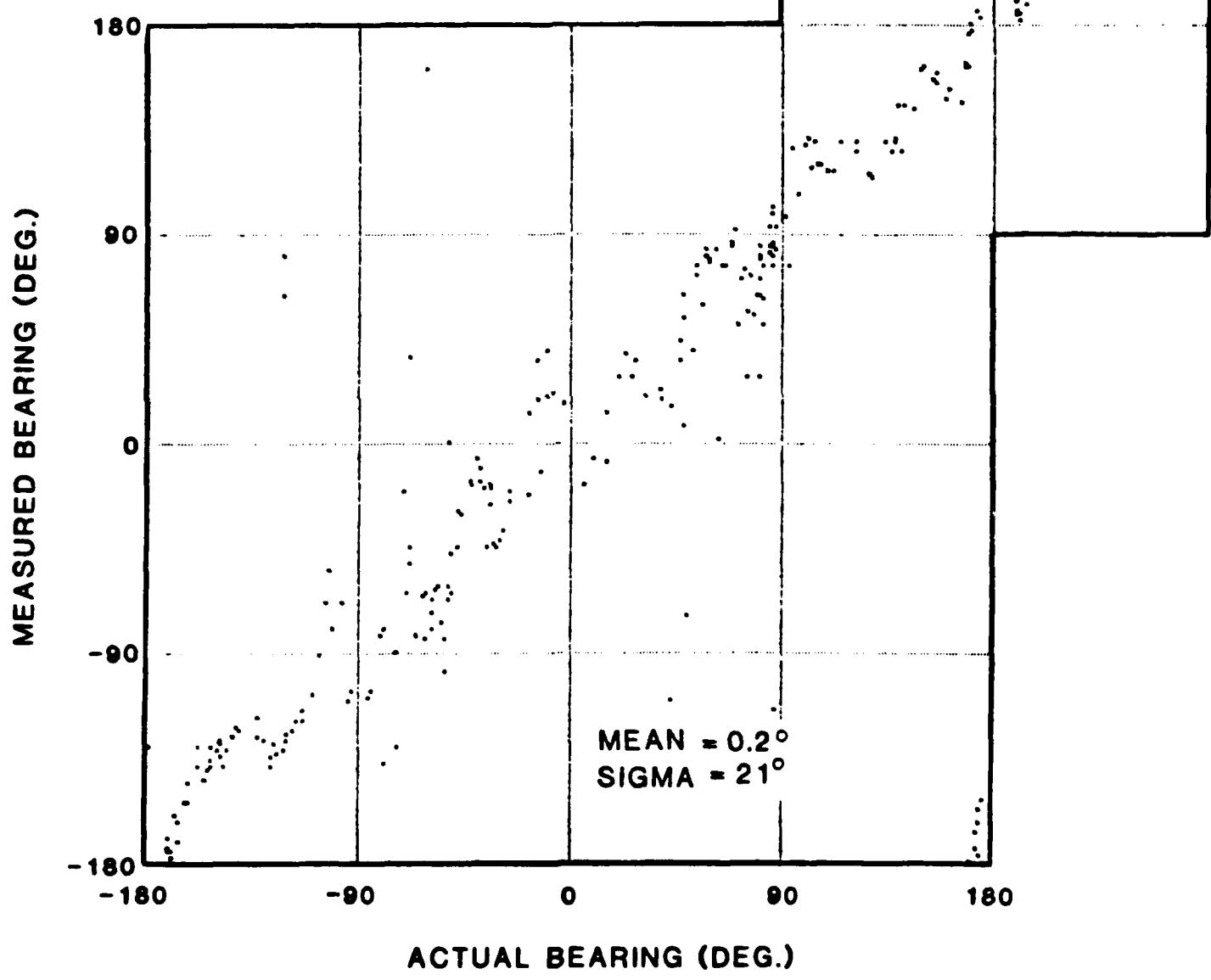
Fig. 4-13. AOA transfer function, helicopter at 500 ft. altitude.
