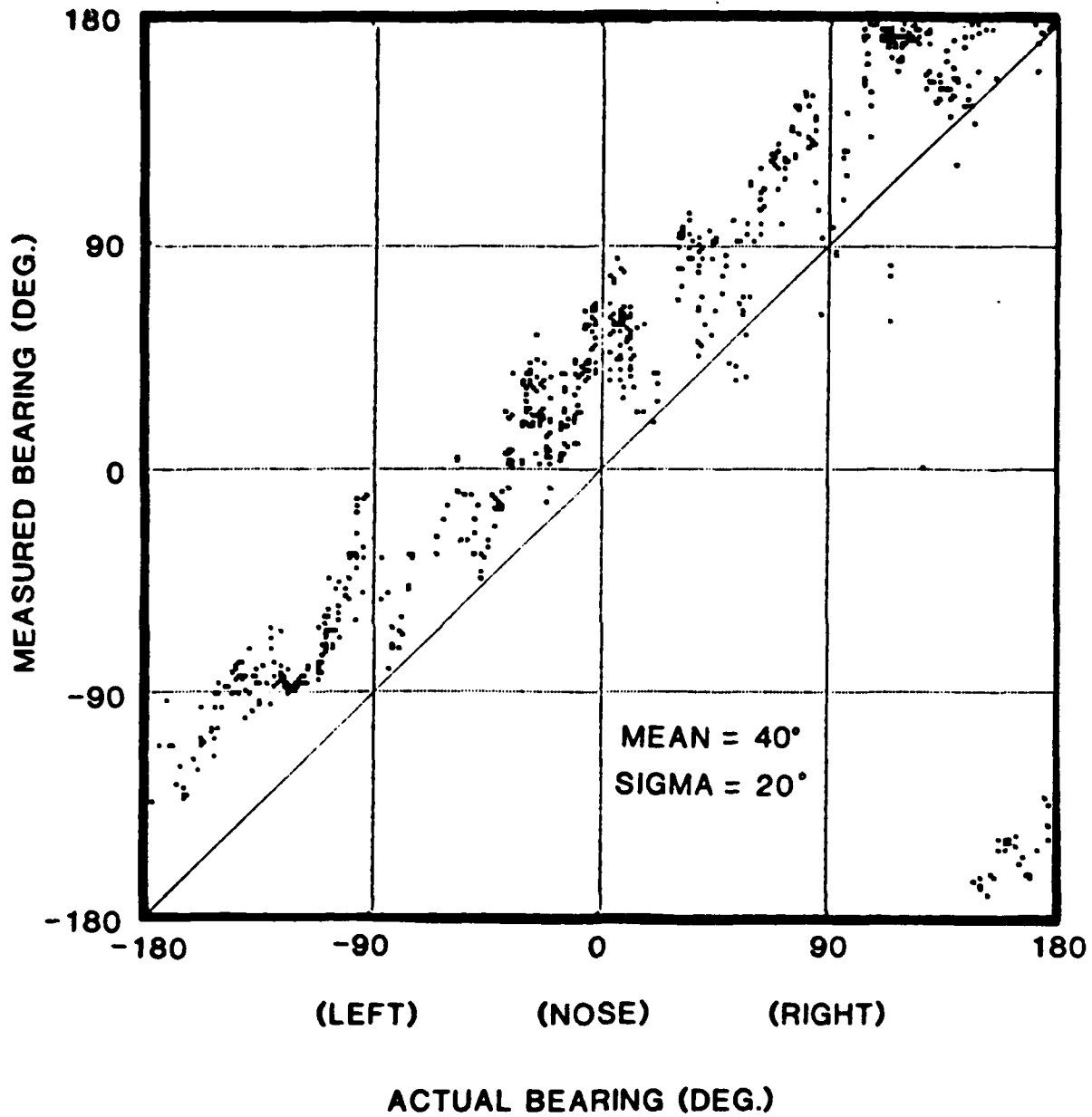
Fig. 4-8. AOA performance hovering just above the ground (30 Nov. 84).
