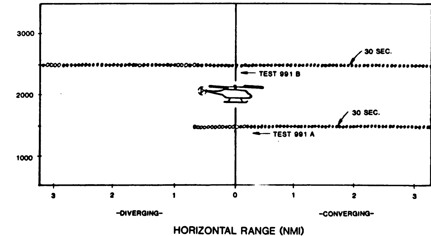
Fig. 3-6. Mode S surveillance performance in head-on encounters.
