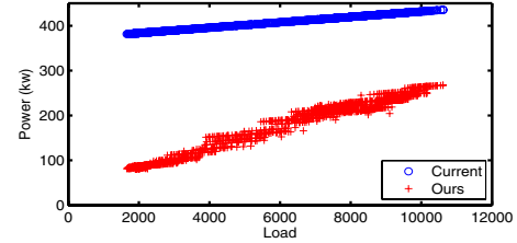
Figure 2: Energy-Load Curve for Region 1 Network.
