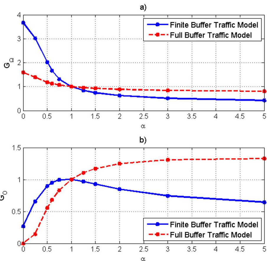
Figure 2 Finite and full buffer traffic models comparison. (a) Average user throughput gain over Proportional Fair G_\alpha . (b) User throughput at 5% outage gain over Proportional Fair G_0 for different \alpha values.
