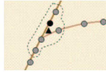
Fig. 6. Identifying the road closest to a certain GPS-provided position. The dots are map points generated from Tiger Line information. The triangle represent the GPS position. The dots in the enclosure are the map points that have the closest simple Peano keys to the simple Peano key of the GPS position for r=2 . The closest map point to the GPS position is colored black, and its position determines the closest road
