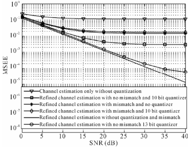
Figure 1. Simulated MSEE as a function of SNR for the proposed channel estimation scheme employing 10 bit and 13 bit channel quantizers [6].
