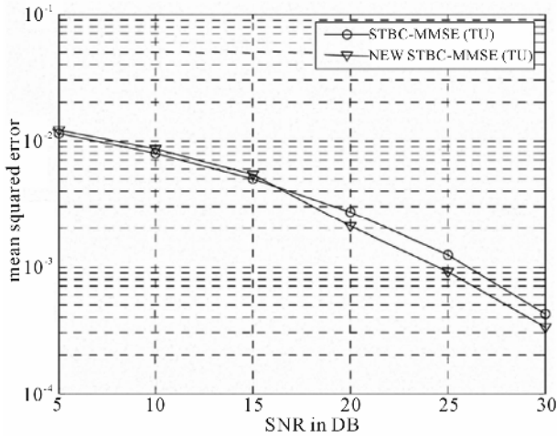
Figure 3. MSE of channel estimators under TU delay profile [8].
