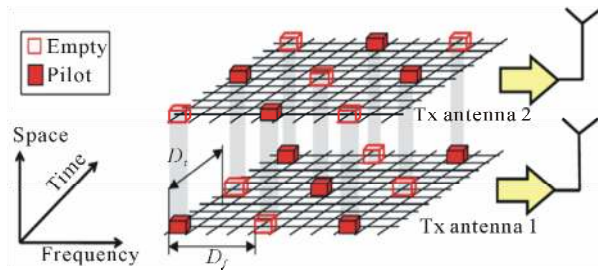
Figure 6. Three dimensional (3D) pilot grid for MIMO-OFDM [14].
