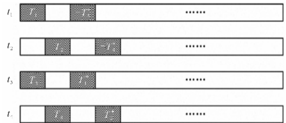
Figure 2. Simplified transmitting pattern of training blocks [8].
