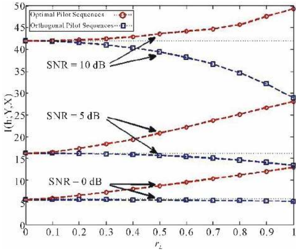
Figure 4. CMI versus r_L without transmit correlation and receive correlation [11].
