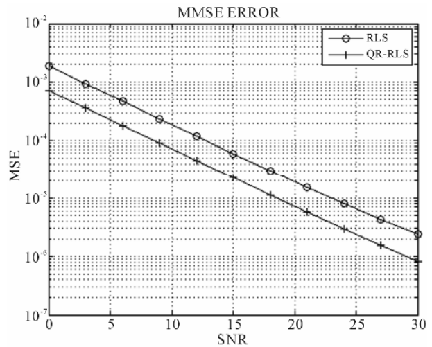
Figure 5. MMSE error for 2 \times 2 MIMO system [13].
