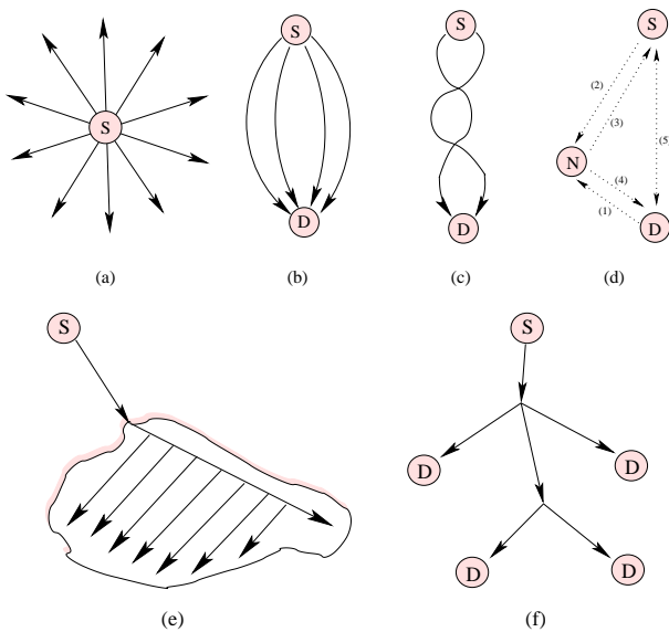
Figure 5: Examples of trajectory routing and forwarding
