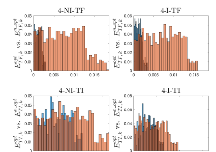
Fig. 5: Case 4: quadrotor – sensitivity of q w.r.t. k_\tau/I . Top row: E_{TF,k}^{opt} (blue histogram) vs. E_{TF,k}^{n-opt} (orange histogram) for the cases 4-NI-TF (left) and 4-I-TF (right). Bottom row: E_{TI,k}^{opt} (blue histogram) vs. E_{TI,k}^{n-opt} (orange histogram) for the cases 4-NI-TI (left) and 4-I-TI (right).
