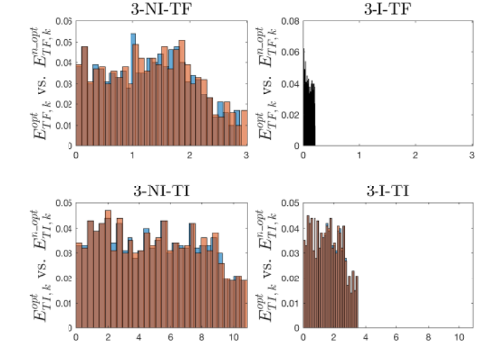
Fig. 4: Case 3: quadrotor – sensitivity of q w.r.t. k_f/m . Top row: E_{TF,k}^{opt} (blue histogram) vs. E_{TF,k}^{n-opt} (orange histogram) for the cases 3-NI-TF (left) and 3-I-TF (right). Bottom row: E_{TI,k}^{opt} (blue histogram) vs. E_{TI,k}^{n-opt} (orange histogram) for the cases 3-NI-TI (left) and 3-I-TI (right).
