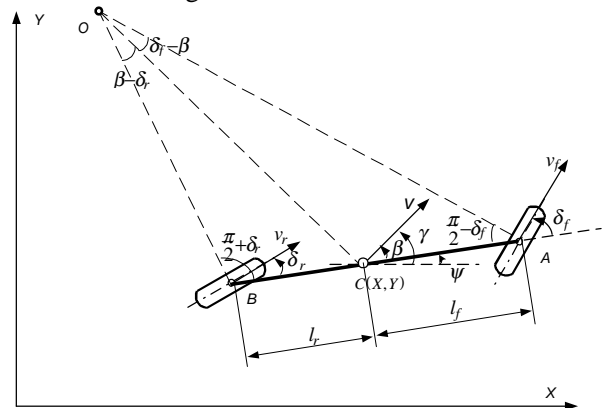
Figure 2 Kinematic model
