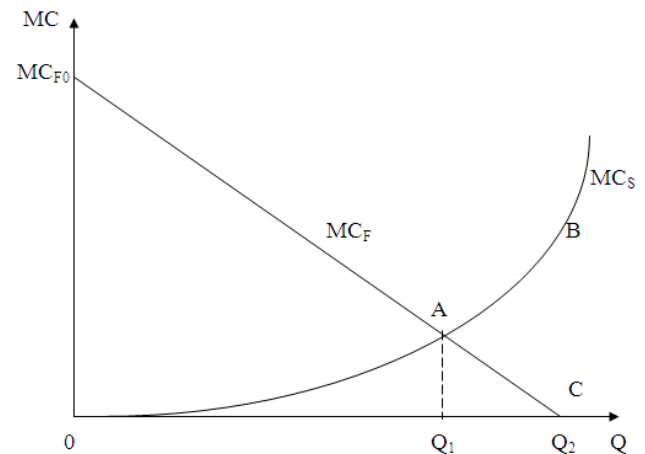
Figure 1. Efficiency of a factory at decrease of contamination environments [12]: MC_F - limiting costs of a factory on decrease of contamination of the environment; MC_S - limiting social costs of contamination for the inhabitants of terrain; Q - value of contamination of the environment
