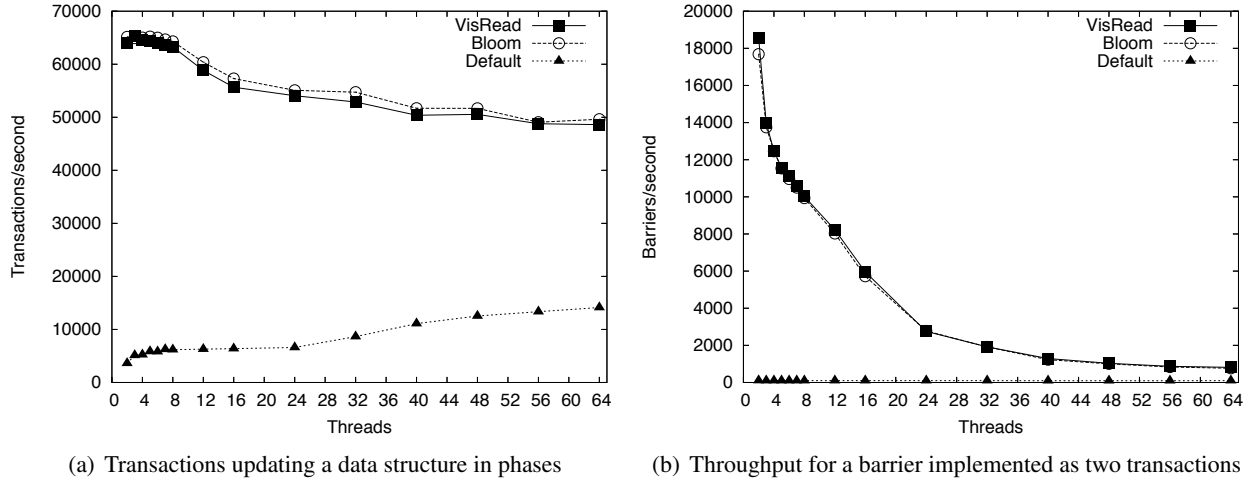
Figure 1: Comparison of Bloom-based retry to optimized visible-reader retry in RSTM. Up to 64 retry transactions are supported via per-object visible reader bitmaps. Bloom filters are configured with 1024 bits and 3 hash functions.
