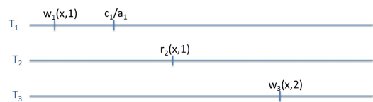
Figure 7. Strictness
