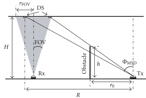
FIGURE 2: MSD architecture: Rx (receiver), Tx (transmitter), DS (diffusing spot), \Phi_{MSD} (maximum transmit semiangle), i_{FOV} (receiver acceptance half angle), r_{FOV} (radius of the circular area in the ceiling that is seen by the receiver), H (communication cell height), R (communication cell radius), h (blocker height), r_0 (minimum possible blocker-portable unit distance).
