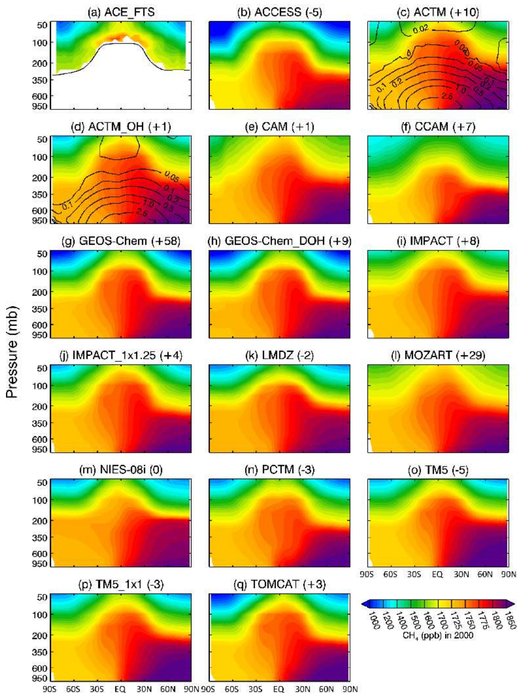
Fig. 3. Annual and zonal mean latitude-pressure (in mb) cross-sections of CH 4 for tropospheric and lower stratospheric altitudes as observed by the ACE-FTS instrument ( a ; climatology) and as simulated by the models in 2000 ( b–o ). The black line in ( a ) shows the climatological tropopause height. The contour lines in ( c and d ) show CH 4 loss rate (units: molecule cm -3 s -1 ) as in the ACTM and ACTM.OH, respectively. An offset is added to the concentrations in each panel (given after the model name in ppb) that adjusts the model fields to a common average value of 1770 ppb between 950 mb and 500 mb. Detailed model-to-model comparisons for 222 Rn, SF 6 , CH 4 and CH 3 CCl 3 for two seasons and over two longitudes are available in the Supplement (Figs. S1–S17).
