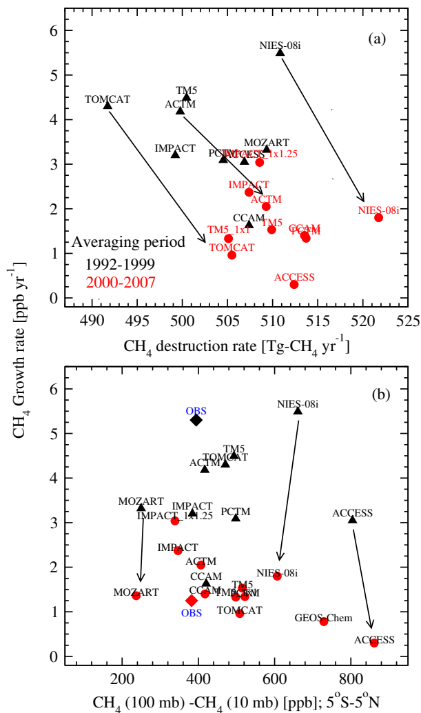
Fig. 11. Relationships of global loss rates for different models (CH 4 EXTRA) with their simulated growth rates at surface sites (a), and the modeled vertical gradients in the lower stratosphere (100–10 mb layer; b) with growth rate. ACTM OH and GEOS-Chem DOH are excluded from this analysis as those models used different OH fields.
