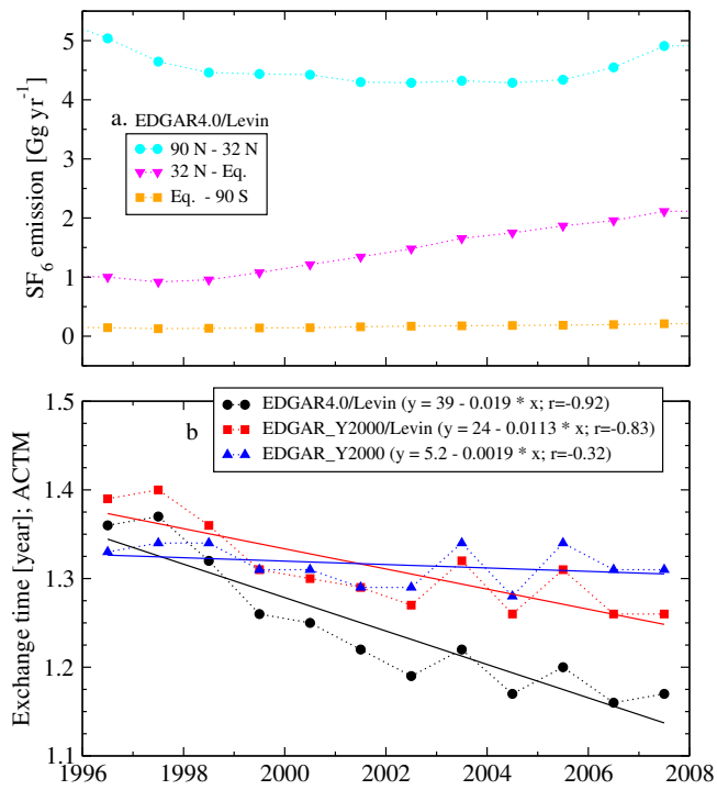
Fig. 9. SF 6 emissions in three broad latitude bands (a, top panel), and \tau_{\text{ex}} (b, bottom panel) estimated using ACTM simulated SF 6 time series for three different emission scenarios.
