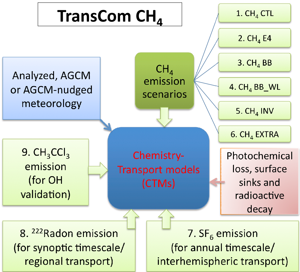
Fig. 1. Schematic diagram of TransCom-CH 4 model simulation experiment.
