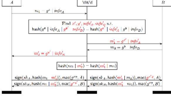
Fig. 2. Man-in-the-middle credential forwarding attack on SIGMA'. The attacker creates a transcript collision by tampering with the messages shown in red. At the end of the protocol, the client and server have seemingly authenticated each other, but the attacker knows both connection keys, and hence can read or write any data.
