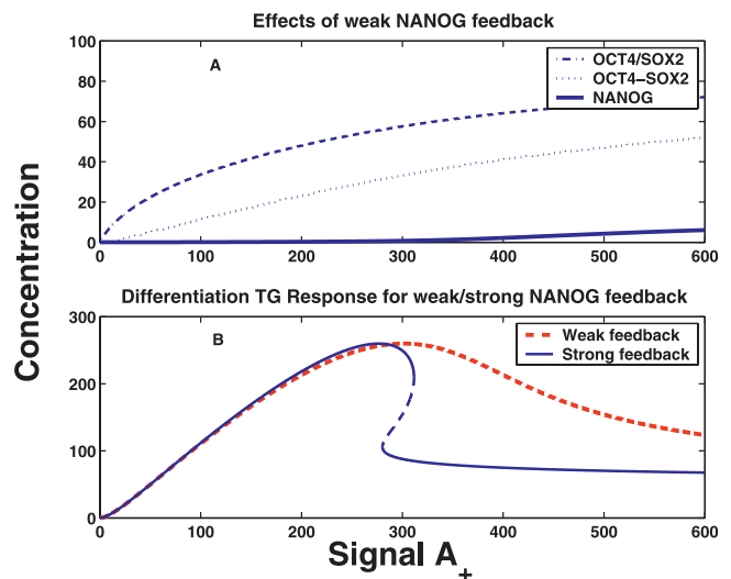
Figure 9. Steady State Values of TG Expression as a Function of the Input Concentration A_+ , for the Differentiation and Sel-Renewal Genes for the Case when NANOG Binds Weakly/Strongly to the OCT4 and SOX2 Genes (A) The effects of weak feedback of NANOG to the OCT4 and SOX2 genes. The inefficient binding of NANOG to these genes leads to a loss of the switch-like behavior. (B) The consequence of weak NANOG binding on the TG expression. With weak feedback, the expression level does not fall off sharply as compared with the case with strong feedback, thereby demonstrating that strong feedback is essential to prevent the differentiation TGs from being expressed.
