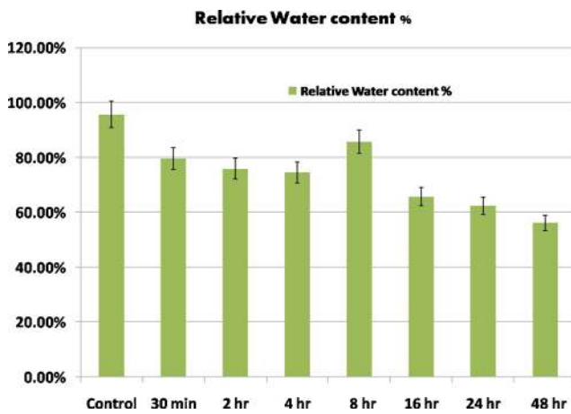
Fig. 1 Variation in Relative Water Content ( RWC ) of drought stressed plants by PEG 6000 from different time duration (A-Control, B-30 min, C-2 h, D- 4 h, E- 8 h, F- 16 h, G- 24 h and H-48 h)
