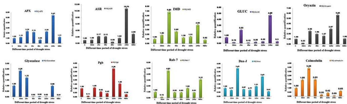
Fig. 6 RT-qPCR analysis of ten drought responsive genes identified in a SSH library of P. glaucum cultivar PPM1741. Relative levels of expression of Abcisic stress ripening protein (Asr) , Ascorbate peroxidase (Apx) , Inosine-5'-monophosphate dehydrogenase(IMD) , Putative beta-1, 3-glucanase (GLUC) , Glyoxalase , Rab7 , Aspartic
