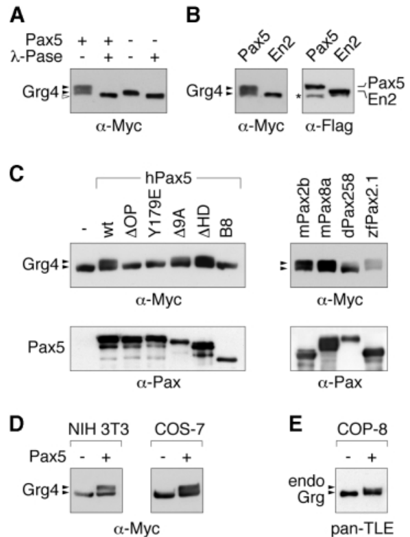
Fig. 6. Induced phosphorylation of Grg4 upon interaction with Pax5. (A) Pax5-dependent phosphorylation of Grg4. Pax5 (where indicated) and Myc-tagged Grg4 were transiently expressed in COP-8 cells for 48 h. Grg4 was then precipitated from whole-cell lysates with a monoclonal anti-Myc antibody, incubated with \lambda protein phosphatase ( \lambda -Pase) and then analyzed by Western blotting with a polyclonal anti-Myc antibody. (B) Specificity of the Grg4 phosphorylation. Myc-tagged Grg4 and Flag-tagged Pax5 or En2 proteins were co-expressed in COP-8 cells followed by Western blot analysis with anti-Myc and anti-Flag antibodies, respectively. The asterisk denotes a cross-reacting protein. (C) The phosphorylation of Grg4 depends on direct interaction with Pax2/5/8 proteins. The Pax proteins indicated were co-expressed with Myc-tagged Grg4 in COP-8 cells followed by Western blotting with polyclonal anti-Myc and anti-paired domain antibodies. (D) Phosphorylation of Myc-tagged Grg4 in NIH 3T3 and COS-7 cells co-expressing Pax5. (E) Endogenous (endo) Grg proteins are phosphorylated in Pax5-expressing COP-8 cells, as shown by Western blot analysis with a pan-TLE (Grg) antibody (Stifani et al. , 1992).
