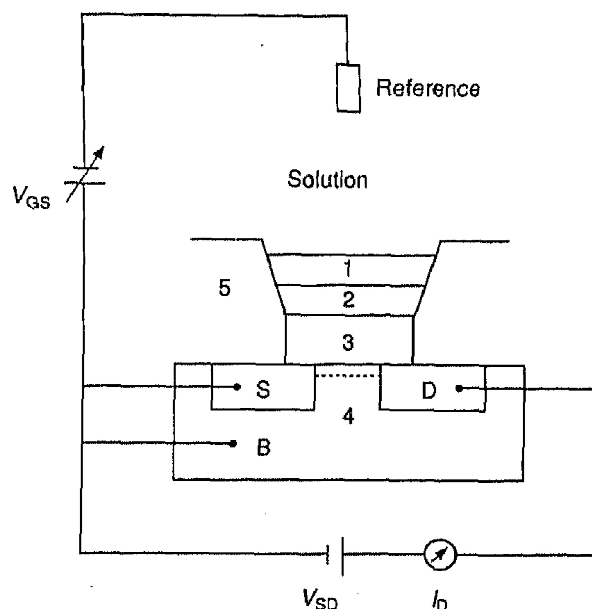
Fig. 1 Scheme of a chemically modified field effect transistor (CHEMFET)
