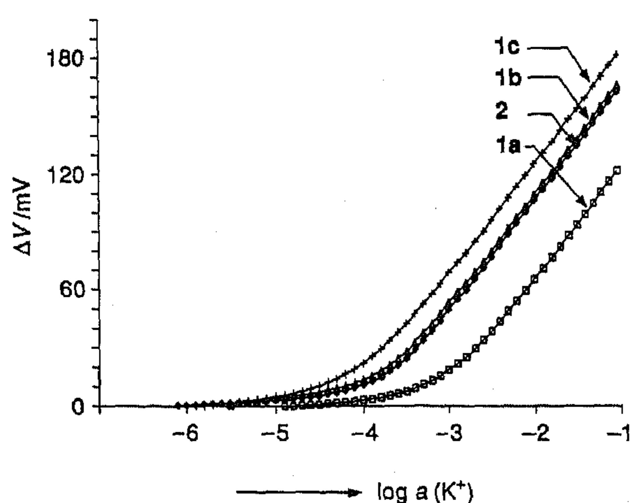
Fig. 3 K^+ responses of CHEMFETs based on PVC membranes containing ionophores 1a-c and 2 ( 0.10 \text{ mol dm}^{-3} sodium chloride)
