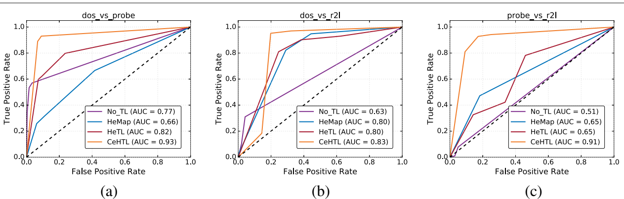
Fig. 6 Performance comparison of ROC curves on the three transfer learning datasets. a ROC curve on DoS→Probe. b ROC curve on DoS→R2L. c ROC curve on Probe→R2L
