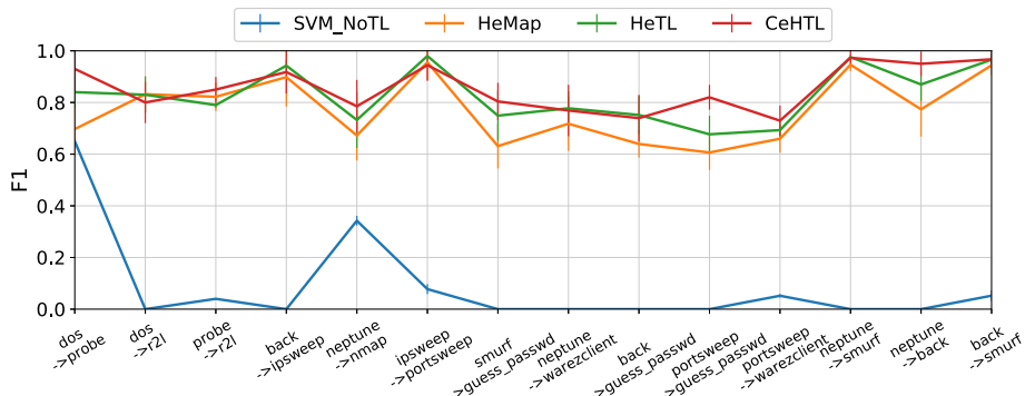
Fig. 5 Performance comparison of F_1 score on unknown network attacks detection, sample size = 1000
