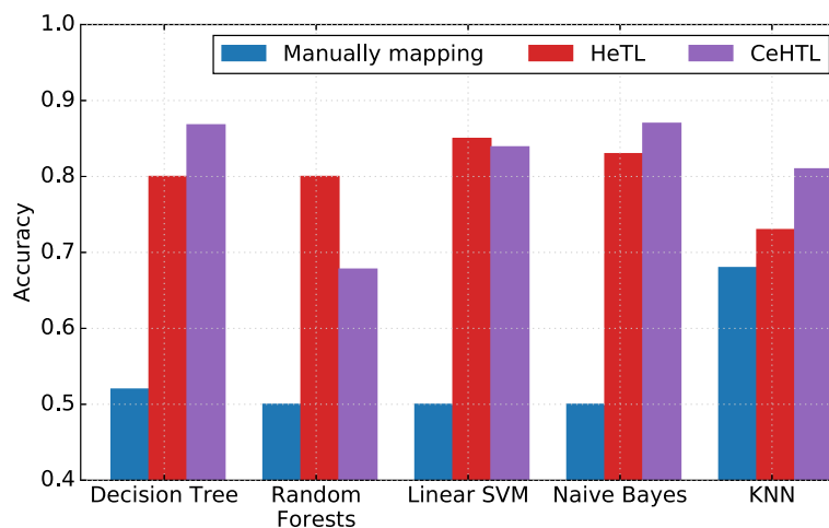
Fig. 8 Performance comparison on heterogeneous spaces on DoS → R2L
