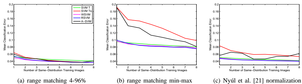
Figure 7. Learning curves for WML/MSL segmentation, showing mean classification error as a function of the number of T_s samples on 13 features for three different normalization techniques. (a) equals the image in Fig. 5(b) and includes range matching between the 4th and 96th percentile, (b) includes range matching between the minimum and maximum value, and (c) includes the normalization of Nyúl et al. [21].
