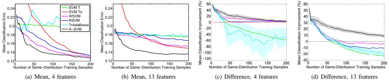
Figure 2. Learning curves showing the mean classification error and classification improvement on the test sets as a function of the number of T_s samples, for the six classifiers: an SVM on T , an SVM on T_s , WSVM, RSVM, TrAdaBoost, and A-SVM. (a) and (b) show the average learning curves over all 56 images from the four sources, for 4 and 13 features respectively. (c) and (d) show the percentage reduction in mean classification error compared to the SVM T_s classifier, averaged over all 56 images, for 4 and 13 features respectively. For TrAdaBoost and A-SVM 95%-CIs for the mean improvement were included, the CIs of SVM T , WSVM, and RSVM were similar to the CI of A-SVM.
