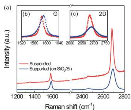
Figure 5. (a) Raman spectra of monolayer graphene on flat \text{SiO}_2/\text{Si} and perforated silicon nitride supporting film using a 514 nm wavelength laser. (b) Raman spectra of G-band region ( 1520\text{--}1640 \text{ cm}^{-1} ). (c) Raman spectra of 2D-band region ( 2600\text{--}2750 \text{ cm}^{-1} ).
