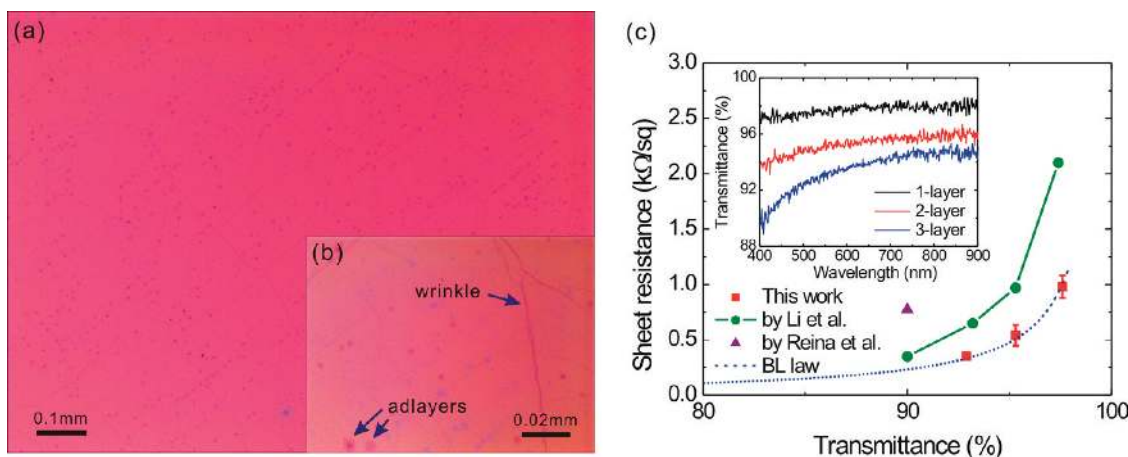
Figure 6. Evaluation of graphene films transferred onto flat substrates. (a, b) Optical images of large-area monolayer graphene transferred onto 285 nm \text{SiO}_2 : (a) field of view 1.2 \text{ mm} \times 0.9 \text{ mm} and (b) field of view 0.12 \text{ mm} \times 0.09 \text{ mm} . (c) Sheet resistance as a function of transmittance at \lambda = 550 \text{ nm} . The squares are the results from graphene transferred to glass slides by this method. The circle and triangle represent CVD-grown graphene grown on copper by Li et al. 20 and nickel by Reina et al. , 58 respectively. The blue dotted line represents the Beer–Lambert law (indicated as “BL law”) fitted to results from this work. The inset is the transmittance of our n -layer graphene films as a function of wavelength of the incident light with a blank coverslip used for background subtraction.
