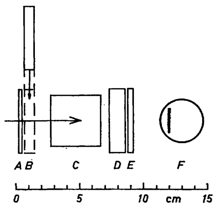
Fig. 1. Schematic diagram of experimental arrangement for measuring relative luminescence intensities. (A) Light filter (Schott UG2, 2 mm). (B) Uranyl glass. (C) Cylindrical glass cell, 4 \times 4 cm. (D) Quartz cell with 0.5 M sodium nitrite solution. (E) Light filter (Chance OY3, 4 mm). (F) Multiplier phototube, RCA 931 A. — A light-tight box with an opening for the exciting beam enclosed parts C–F. The measurements were made in a darkened room.
