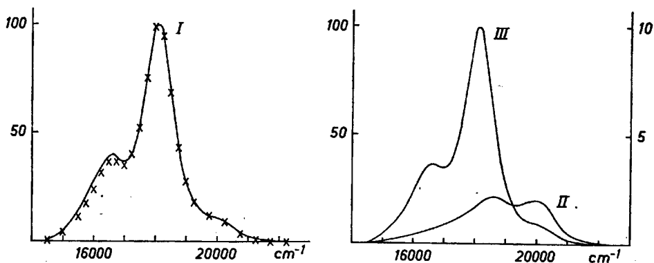
Fig. 6, a and b. Luminescence spectra of anisil. (I) Unsensitized luminescence. Anisil 6.9 \times 10^{-2} M, observed values. (X) Calculated values. (II) Fluorescence (scale to the right). Anisil 1.27 \times 10^{-2} M, pyrene 2.7 \times 10^{-4} M. (III) Sensitized luminescence (scale to the left). Benzophenone 2.64 \times 10^{-3} M, anisil 7.8 \times 10^{-4} M.
