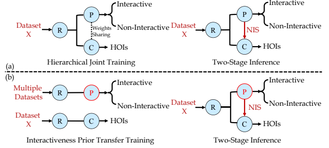
Figure 6. The schemes for training and testing. (a) In Default Mode , \mathbf{P} and \mathbf{C} are first trained jointly with weights sharing on the same dataset. (b) In Transfer Learning Mode , \mathbf{P} can learn interactivenss knowledge across datasets and cooperates with multiple \mathbf{C} s trained on different datasets. In testing, our framework infers in two stages, i.e. \mathbf{P} performs interactivenss discrimination at first, then \mathbf{C} classifies the remaining edges/pairs.
