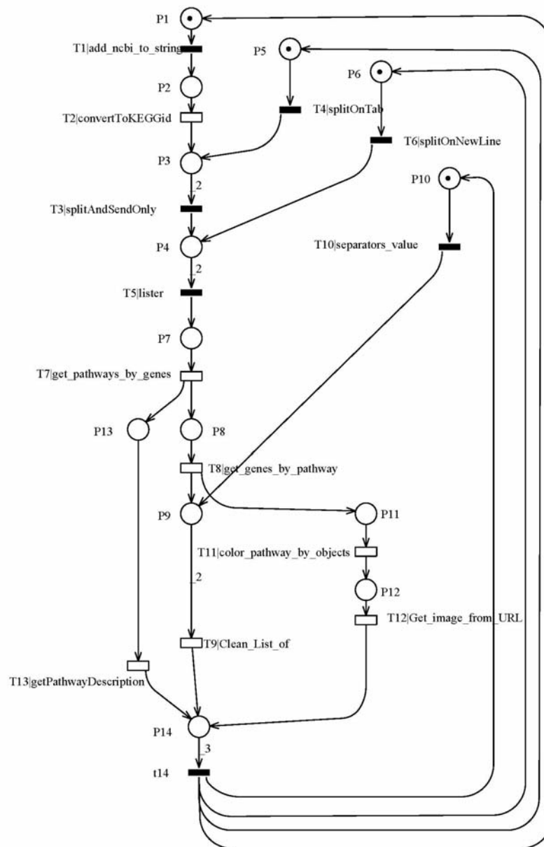
Figure 20. GSPN Pmodel for the GPGE Workflow
