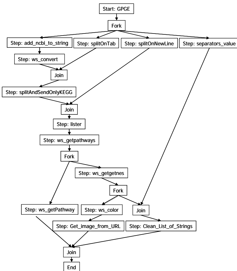
Figure 20. CSM Model of the GPGE Workflow
