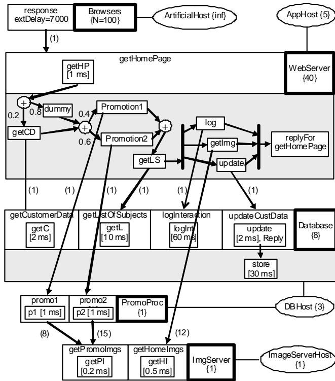
Figure 13. LQN model for the GetHomePage scenario
