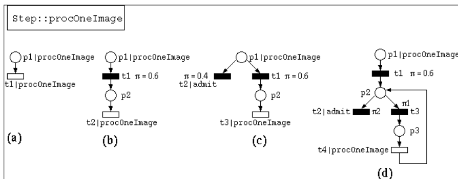
Figure 16. LGSPN patterns for a Step
