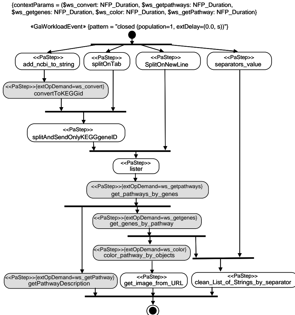
Figure 18. Annotated Activity Diagram for the GPGE Workflow
