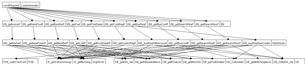
Figure 14. The LQN model created by merging sub-models for ten TPC-W scenario
