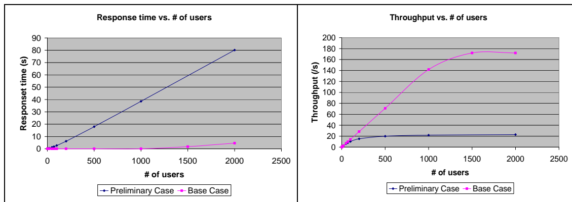
Figure 15. Results for the “preliminary case” with limited concurrency, and the improved “base case”
