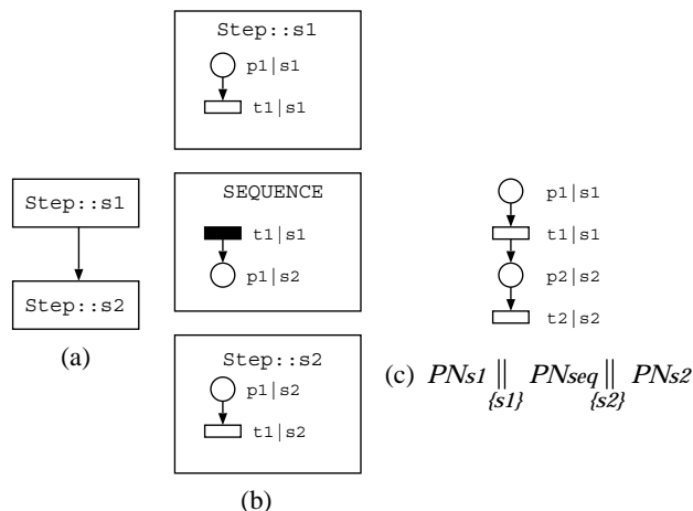
Figure 17. LGSPN patterns for Sequence, and for composing it
