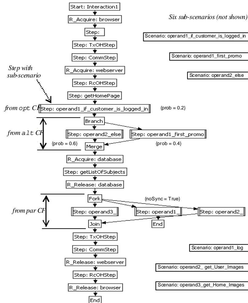
Figure 11. CSM for the GetHomePage Scenario, excluding resources.
