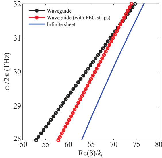
Figure 3.5: Dispersion relation for a graphene nanoribbon waveguide of width w = 200 nm.
