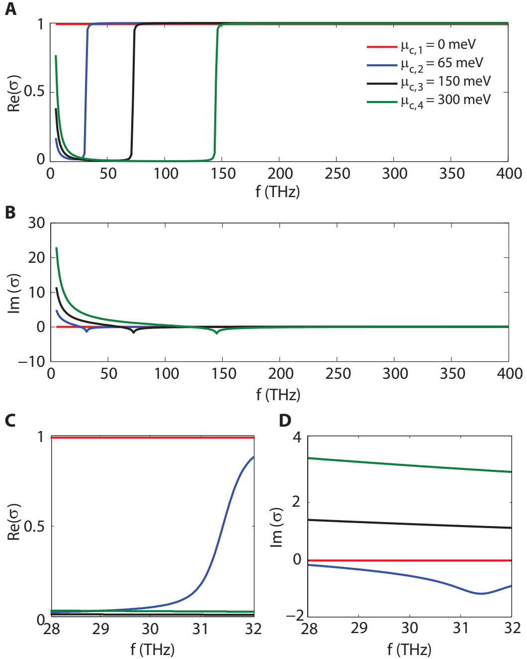
Figure 2.2: Complex conductivity as a function of frequency for different values of chemical potential at T = 3^\circ \text{K} normalized to \sigma_{\min} = \frac{\pi e^2}{2h} . Panels A and B show the real and imaginary part of conductivity for the frequency range 5 to 400 THz, while panels C and D display the portion of mid infra-red region in which we are interested.
