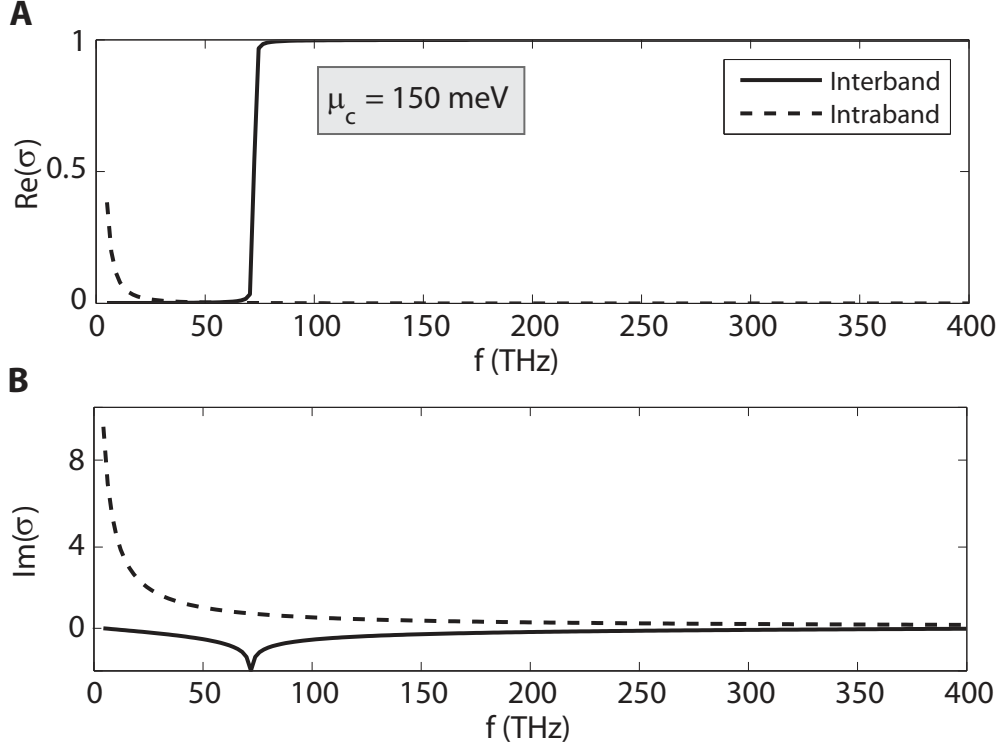
Figure 2.3: Contribution of inter- and intra-band transitions to graphene conductivity for \mu_c = 150 \text{ meV} and T = 3^\circ \text{ K} . Values are normalized to \sigma_{\min} = \frac{\pi e^2}{2h} . Clearly the intraband contribution has the familiar form of Drude, while the interband transition results in higher real part of conductivity for sufficiently high energies (i.e., higher losses for higher frequencies).
