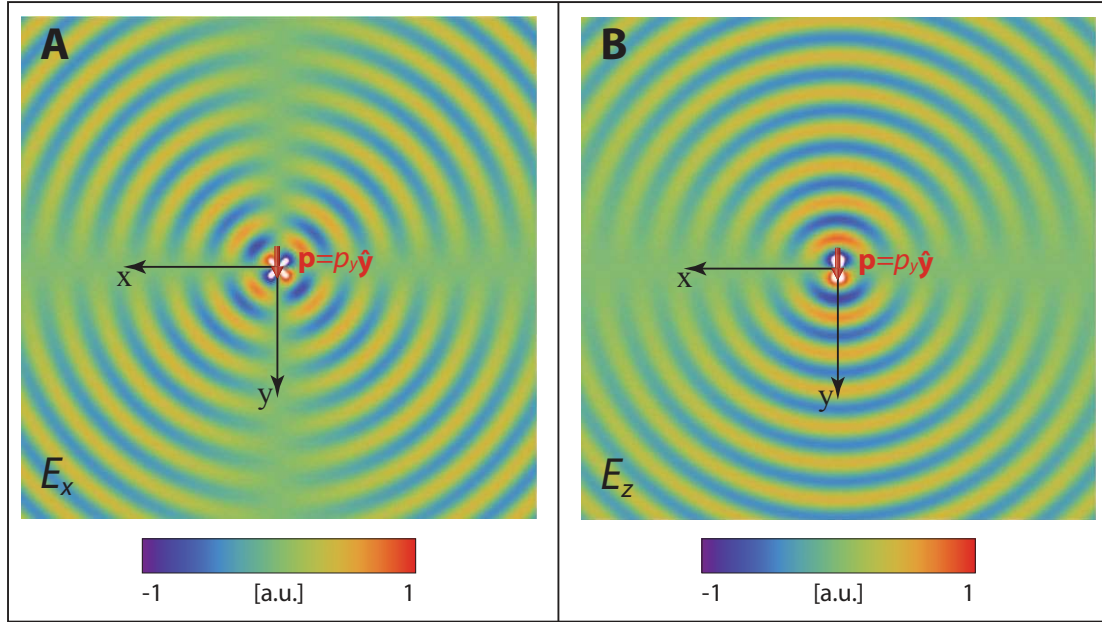
Figure 2.14: The snapshot in time of distribution of E_x and E_z on the plane of graphene due to a horizontal electric dipole on the graphene layer and aligned with y -axis.
