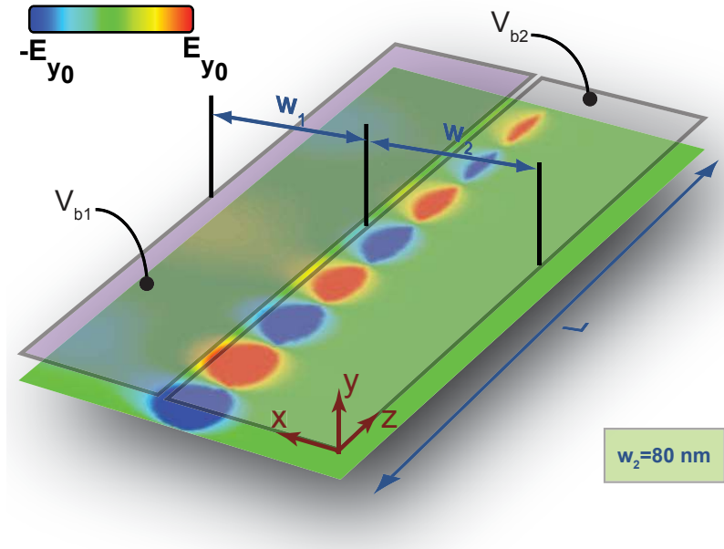
Figure 2.16: Distribution of E_y (snap shot in time) for a guided IR edge wave at f = 30 THz, supported along the boundary line between the two sections of the same sheet of graphene, which has two different conductivity regions ( \sigma_{g,1} = 0.0009 + i0.0765 mS, \sigma_{g,2} = 0.0039 - i0.0324 mS, L = 250 nm, w = 80 nm). Reprinted from Ref. 107 (by permission of the AAAS). [ http://www.sciencemag.org/content/suppl/2011/06/08/332.6035.1291.DC1/Vakil-SOM.pdf ].
