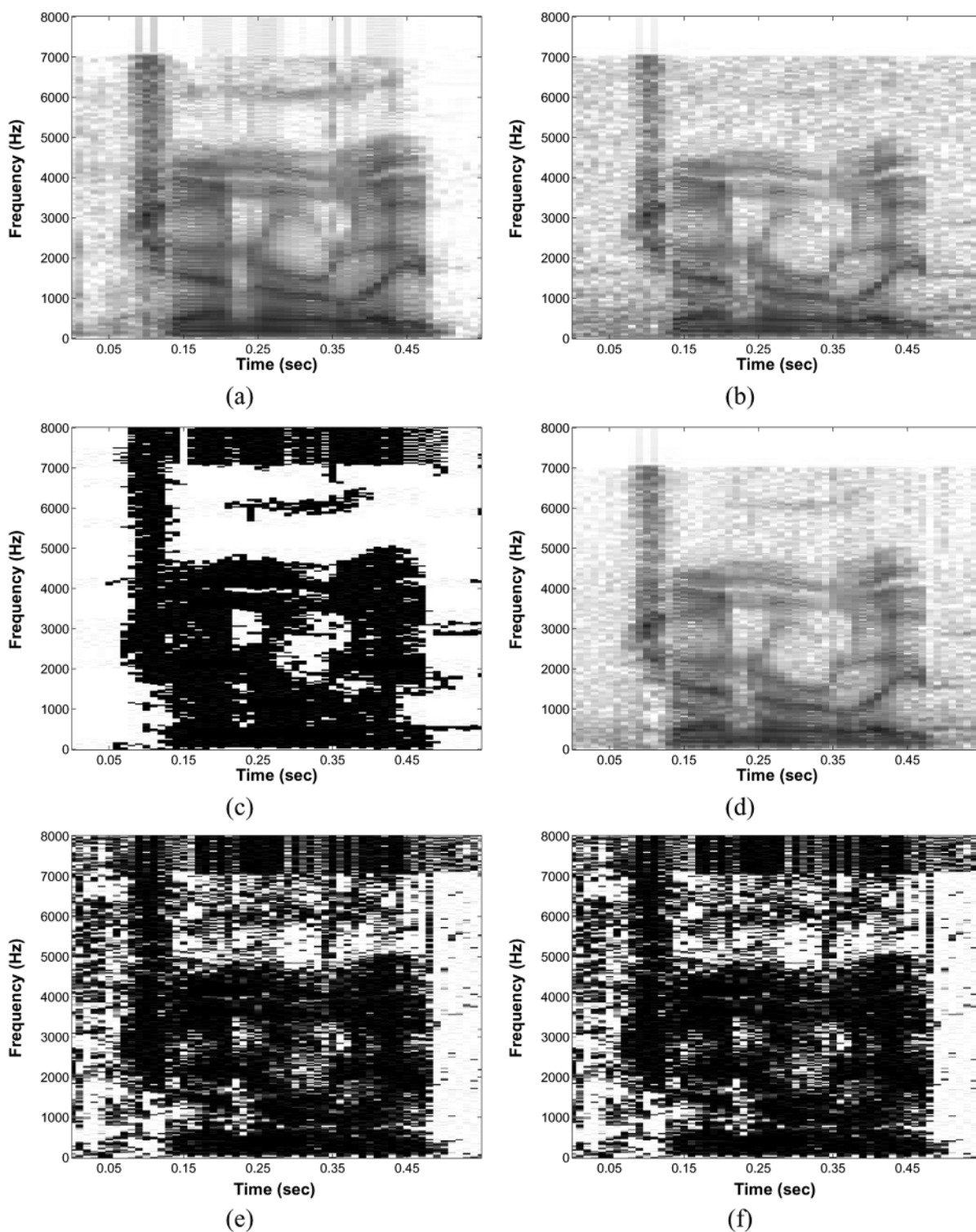
Fig. 2. Comparison between estimated and ideal uncertainties of the reconstructed spectra. (a) The spectrogram of a clean speech utterance. (b) The spectrogram of a mixture of the clean speech utterance and restaurant noise. (c) The binary T-F mask produced by spectral subtraction. Reliable T-F units are marked black and unreliable white. (d) The spectrogram obtained from (b) by applying the mask in (c) followed by reconstruction of the unreliable T-F units. (e) The true uncertainty associated with the reconstructed spectrogram in (d). (f) The corresponding estimated uncertainty.
