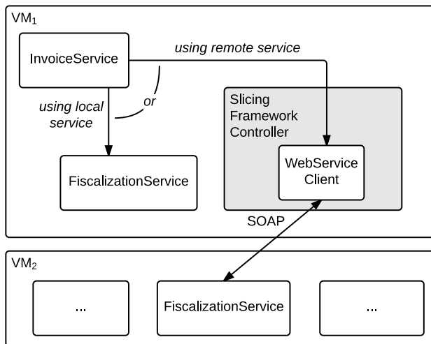
Fig. 6: Framework can use local or remote service
