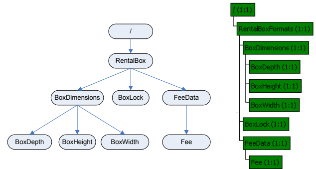
Figure 3 Two visual representations of the same XML schema tree. “Regular” representation on the left. “Flattened” representation on the right.
