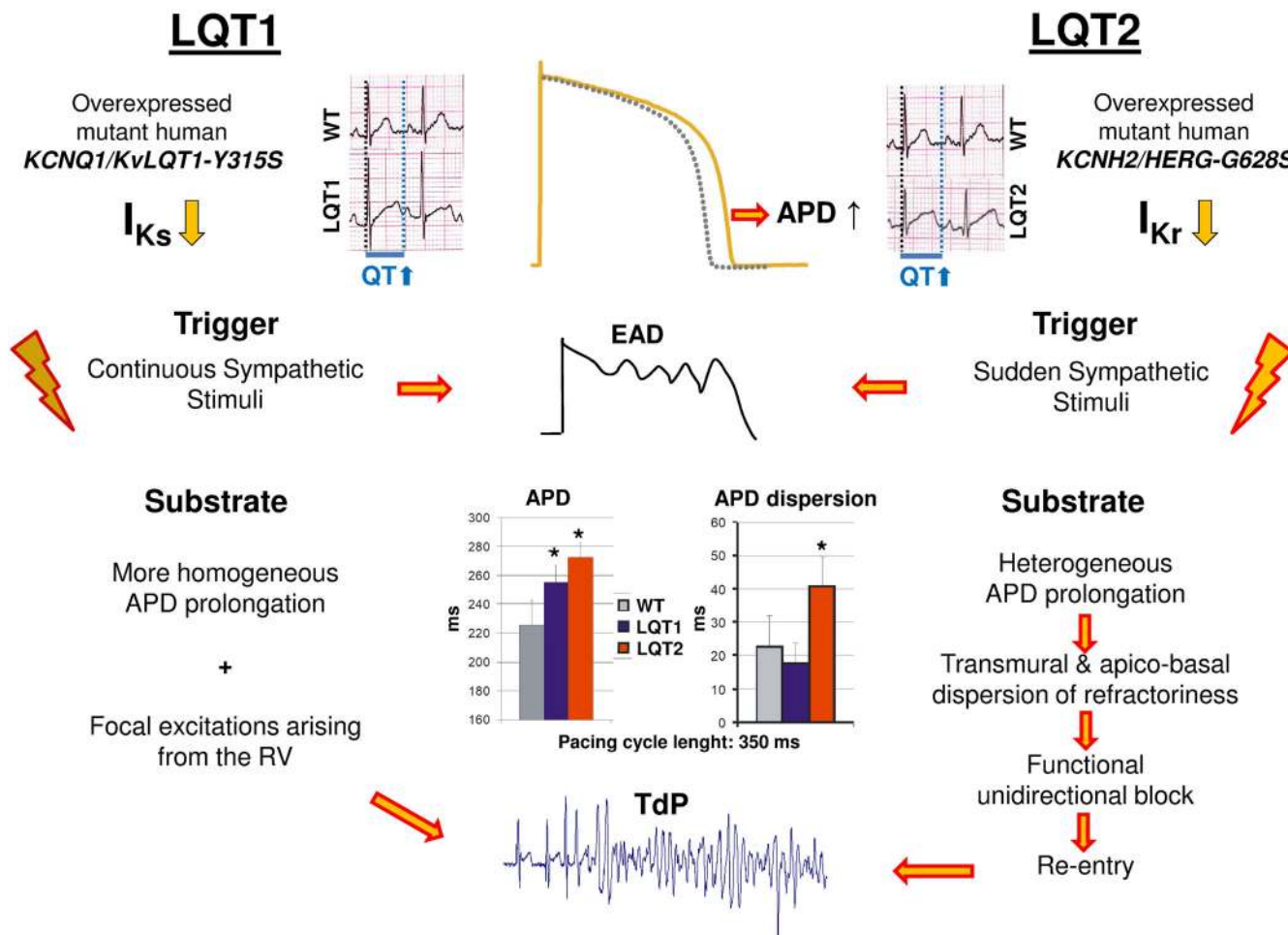
FIGURE 3 Differential arrhythmia mechanisms in transgenic LQT1 and LQT2 rabbits. Schematic illustration of the different genetic backgrounds leading to action potential duration (APD)/QT prolongation (due to loss of I_{Ks} or I_{Kr} ) and differential arrhythmia initiating (trigger) and maintaining (substrate) mechanisms in LQT1 and LQT2 models
