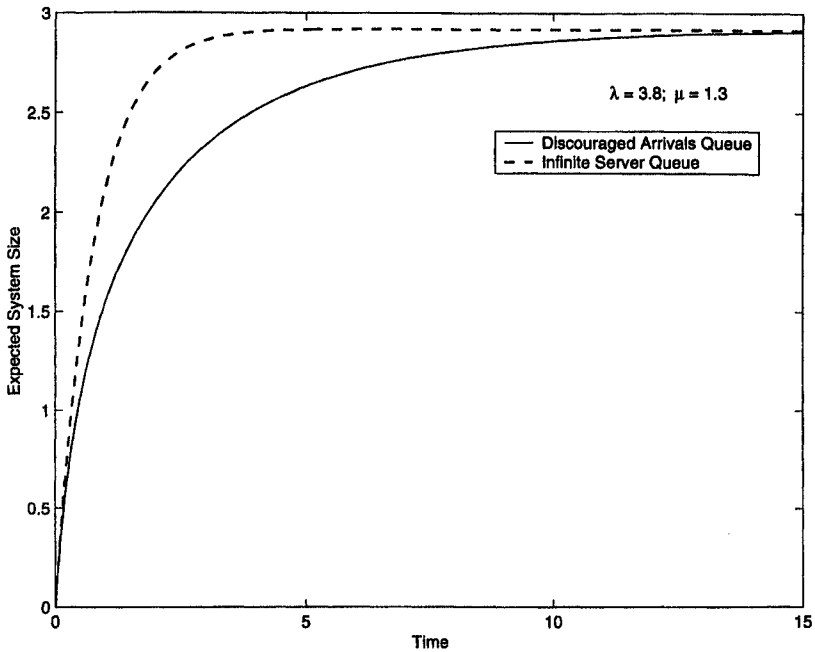
FIGURE 2 Expected system sizes for the discouraged arrivals queue and the infinite server queue.
