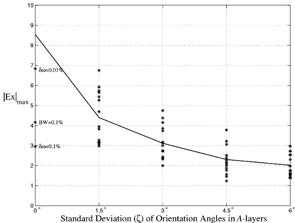
FIG. 14. |E_x|_{\max} inside lossless MPCs with random deviations in the misalignment of A layers. An incidence pulse with BW of 0.01% is considered. For each standard deviation, 15 realizations are produced, leading to the results indicated by the star symbols. The average results for each standard deviation are interpolated by the solid line. Results for incident pulses with incident pulse with \delta\omega=0.01\% (for BW=0.01\% ), \delta\omega=0.1\% (for BW=0.01\% ), and BW=0.1\% (for \delta\omega=0\% ) are also displayed for reference.
