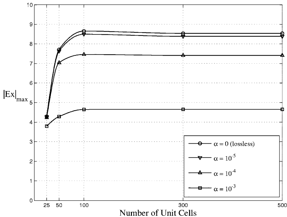
FIG. 13. |E_x|_{\max} inside MPCs with different numbers of unit cells and ferromagnetic loss parameters. Four loss parameters, \alpha=0 , 10^{-5} , 10^{-4} , 10^{-3} , and five different numbers of unit cells (25, 50, 100, 300, 500) are considered.
