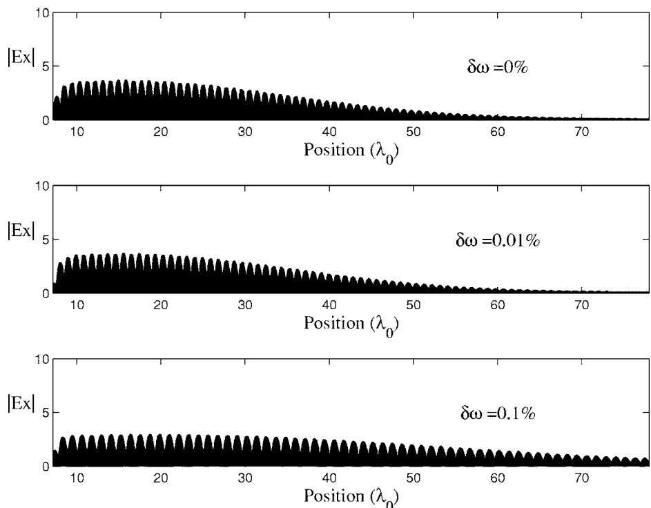
FIG. 9. Snapshots of |E_x| inside the MPC at time step 12 \times 10^6 , with L_F=1.0833 mm. In this case, \Delta t=0.272 ps and \lambda_0=76.733 mm. The top plot indicates the matched-frequency case \delta\omega=0\% , the center plot indicates the frequency-shifted case \delta\omega=0.01\% , and the bottom plot indicates the frequency-shifted case \delta\omega=0.1\% . Note the reduced frequency sensitivity in |E_x| compared to the responses shown in Figs. 3, 6, and 7.
