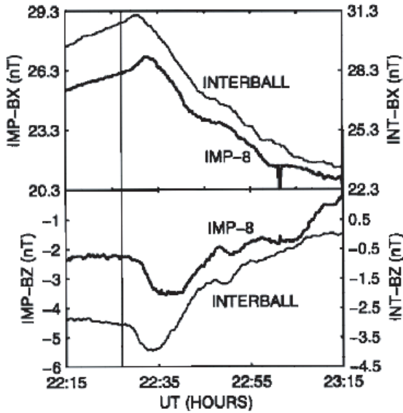
Fig. 15. Tailward propagation of a cross-tail current disruption as evidenced by simultaneous magnetic field measurements taken in the lobe onboard Interball-Tail and IMP-8, separated by about 10 R_E along the X axis of the tail. (From Jacquey et al., 1998).
