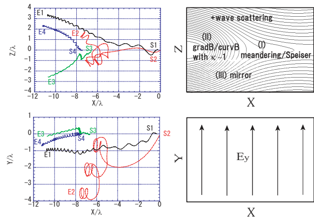
Fig. 43. Several electron trajectories in the reconnection region. (From Hoshino et al., 2001).
