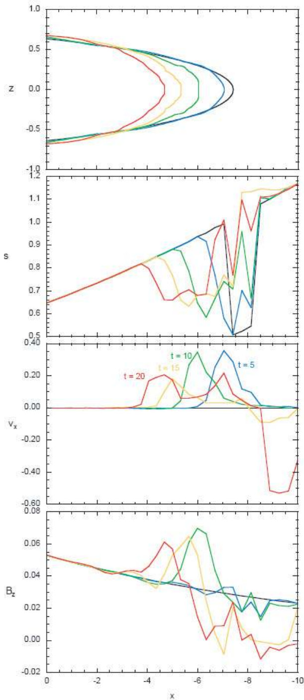
Fig. 38. Evolution of plasma-depleted tube with time in the numerical simulation of a plasma bubble. The bubble is easier to identify based on the depletion the entropy function s=p^{1/\gamma}/\rho . The upper panel shows the motion and reconfiguration of flux tube at the inner edge of the bubble. Other panels show the evolution of entropy, flow velocity and magnetic field B_z -component in the equatorial plane. T=20 corresponds to approximately 8 min of real time. (From Birn et al., 2004).
