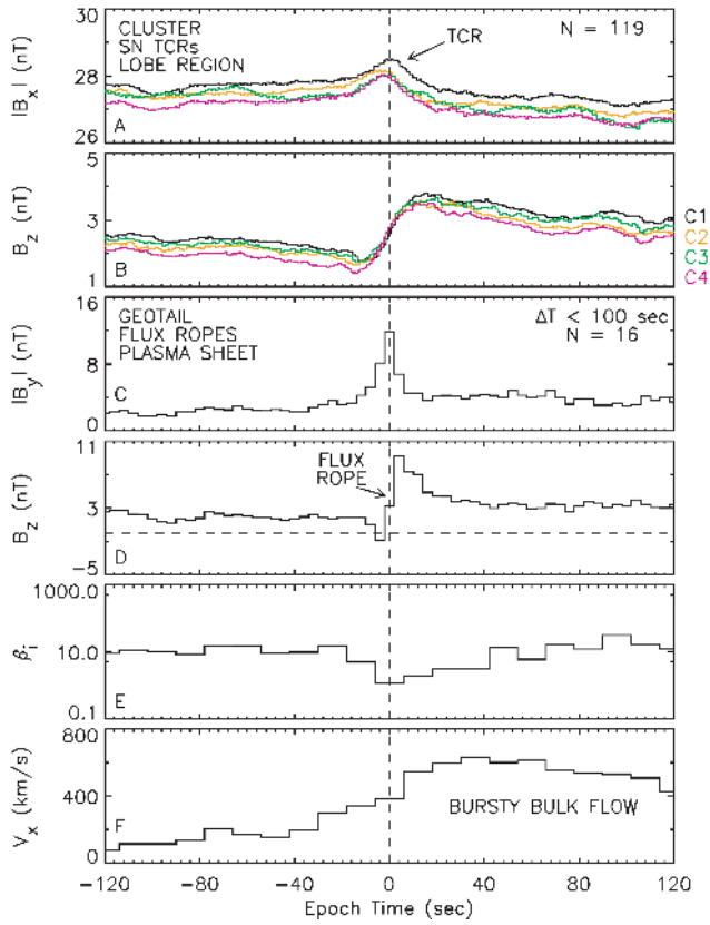
Fig. 9. Merged superposed epoch analyses of Cluster SN TCRs and Geotail BBF-type flux ropes. (From Slavin et al., 2005).
