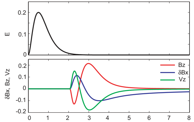
Fig. 29. Variations of the reconnection rate (top) and the corresponding disturbances of \delta B_x = B_x - B_0 , B_z and v_z observed by an artificial spacecraft at the point x=1 , z=.5 in the inflow region (bottom). Magnetic field is normalized to B_0 , velocity to Alfvén velocity v_A , time to the duration of the pulse t_0 , and distance to v_A t_0 .
