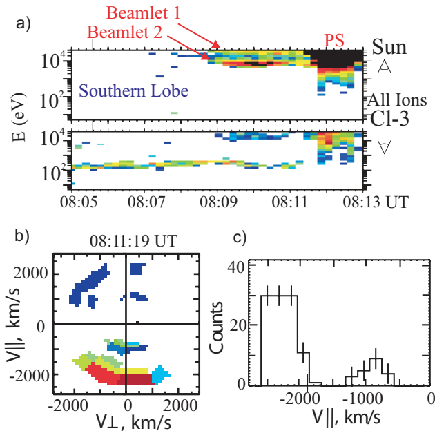
Fig. 25. Cluster observation of “double-peaked” ion distributions in the PSBL on March 9, 2001. E-T spectrograms of Earthward and tailward moving ions obtained by Cluster/HIA (a). 2-D (cut in V_{||}-V_{\perp} plane, b) and 1-D (cut along magnetic field, c) 12 s accumulated ion distribution. (From Zelenyi et al., 2006).
