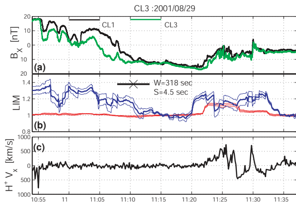
Fig. 47. The magnetic field component B_x measured by Cluster 1 and 3 spacecraft on 29 August 2001 and the local intermittence measure (LIM) from C3. The current sheet was bifurcated in structure and was subject to flapping between 10:55 and 11:05 UT (Runov et al., 2003b). The B_x components at C1 and C3 (panel a) have similar variations but at different levels. The LIM values for the small-scale (red line) and large-scale (blue) variations differ significantly during the current sheet flapping and bifurcation, indicating weak cross-scale coupling or dominantly coherent features. However, the two measures are close when B_x is quiet or is accompanied by flow bursts, as shown by proton data in panel (c). The latter indicates turbulence, with the expected strong cross-scale coupling. (From Vörös et al., 2003).
