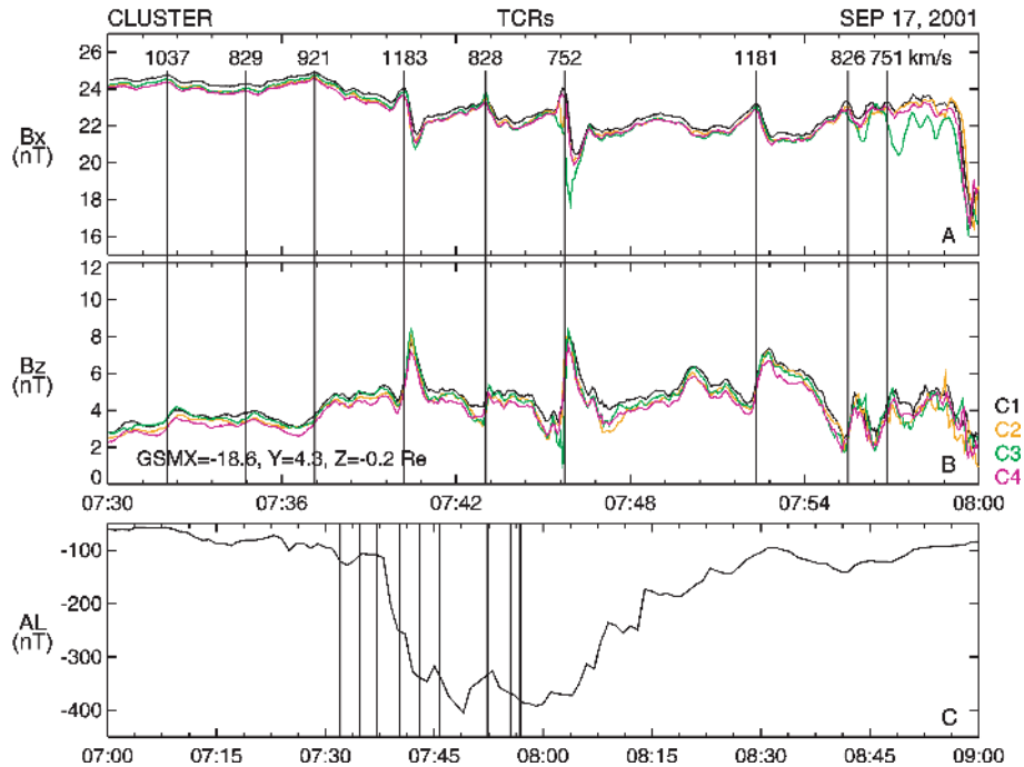
Fig. 7. Example of TCRs observed by Cluster during a substorm on 17 September 2001. The propagation speed of the TCRs, all Earthward, are shown in the top panel. (From Slavin et al., 2005).
