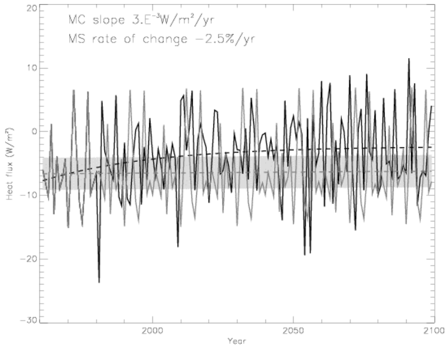
Fig. 2: Time series of the net surface heat flux (in W/m^2 ) integrated over the whole Mediterranean Sea and yearly averaged. In grey, the control run (MC) and in black, the scenario (MS). A linear fit has been computed for MC (grey dashed line) whereas an exponential fit describes MS (black dashed line). The values are the slope of the linear fit for MC and the rate of change (in % per year) of the exponential fit for MS. A range corresponding to a 95% confidence level (in grey) has been added for the fitted curve of MC
