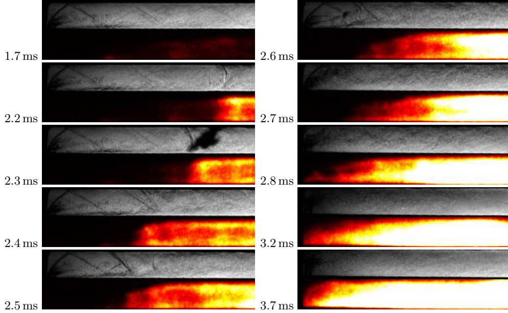
FIGURE 13. Sequence of quasi-synchronous Schlieren and OH* chemiluminescence images of the flow near the injector ( x=56-136 mm) for an equivalence ratio of 1.1.
