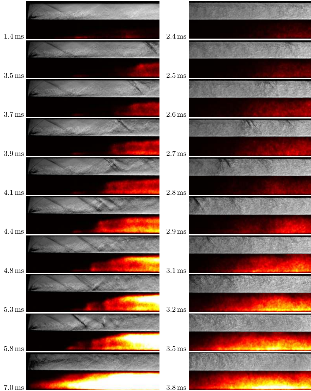
FIGURE 9. Sequences of quasi-synchronous Schlieren and OH* chemiluminescence images of the flow (left) near the injector ( x=56-136 mm) and (right) in the central combustion chamber ( x=158-228 mm) for an equivalence ratio of 0.7.
