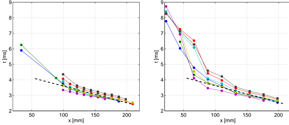
FIGURE 8. X-t diagrams showing the motion of the leading edge of the unsteady shock train in the combustor for an equivalence ratio of 0.7: (left) injector-side wall; (right) cowl-side wall. The dashed line in each case indicates a propagation speed of 93 m/s.
