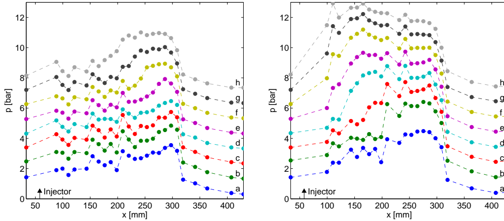
FIGURE 6. Unsteady experimental pressure development inside the combustion chamber for equivalence ratios of (left) 0.5 and (right) 0.7. The measurements are made on the injector-side wall, and are at times (a) 2.4, (b) 2.6, (c) 3.0, (d) 3.4, (e) 3.8, (f) 5.2, (g) 5.6, and (h) 6.6 ms. For clarity, all traces except the first in each plot have been shifted upwards by an integral number of bars.
