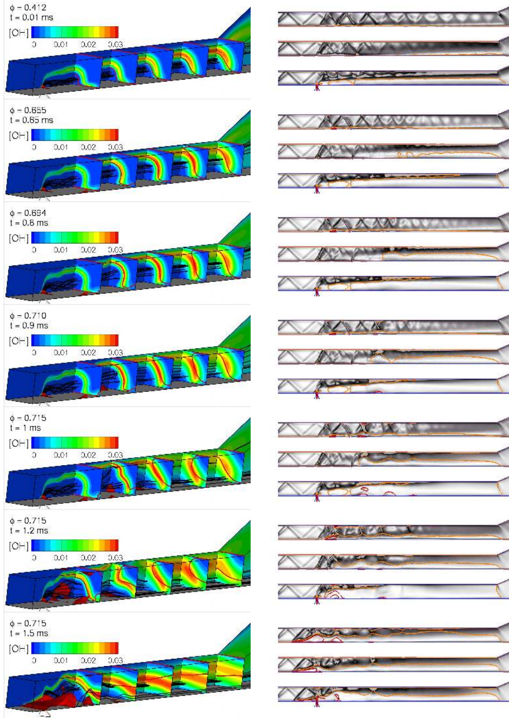
FIGURE 14. Numerical results of the HyShot II combustor choking process at different time instants for a final equivalence ratio of 0.715. To the left are shown contours of OH mass fraction, together with sonic lines (red), streamlines emanating from the injector (black), and boundaries of flow reversal (red surfaces). To the right are shown pseudo-Schlieren images on three equally spaced cut-planes, with sonic lines (orange) and flow reversal boundaries (red) also indicated. The axial coordinate in both cases has been compressed by a factor of two.
