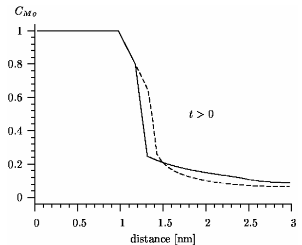
Figure 6: Demonstration of the influence of the 'strength' of the diffusional stress: weak stress – solid line, strong stress – dashed line. (see also Ref. [2])
