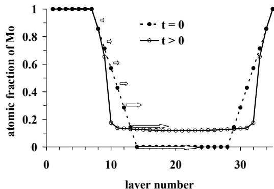
Figure 1: Composition distribution during intermixing in one period of a Mo/V multilayer calculated from an atomistic model, as in [1]. The arrows represent schematically the 'flux distribution', i.e. their lengths are proportional to the absolute value of the atomic flux.
