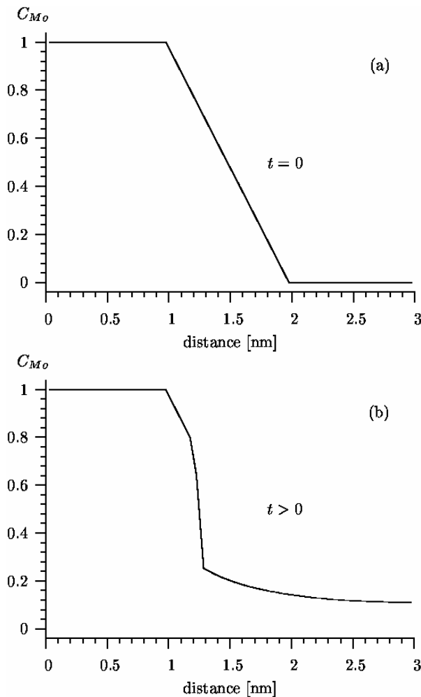
Figure 4: Time evolution of the composition profile of Mo, at two different times, when all the stress effects are ignored. (see also Ref. [2])
