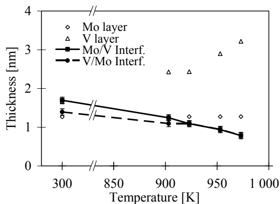
Figure 3: Thickness of the interfaces as well as the pure Mo and V layers, as obtained from the fits. Error bars show the estimated errors of fitting. In case of the pure Mo and V layer, respectively, error bars are comparable to the symbol sizes. The solid curves are to guide the eye.
