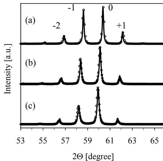
Figure 2: Diffraction patterns measured (circles) during the heat treatments and their reconstructions by the modified Stearns model (solid line): (a) room temperature, (b) 903 K, and (c) 953 K.
