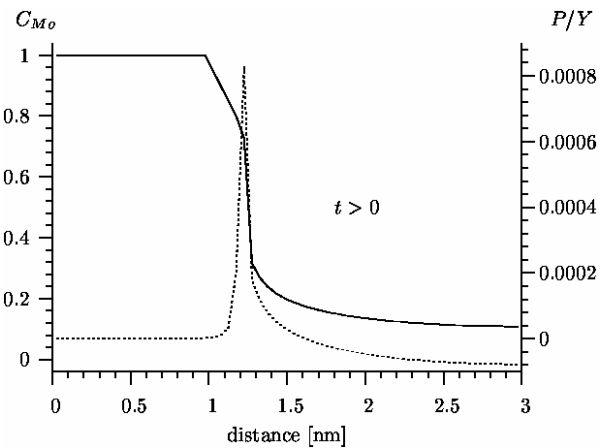
Figure 5: Time evolution of the composition profile of Mo at t > 0 when only the diffusional stress is taken into account (The initial state is the same as in Fig. 4a). The dotted line is the normalised pressure [P/Y where Y = E/(1-\nu) , E Young's modulus, \nu Poisson's ratio] (see also Ref. [2])
