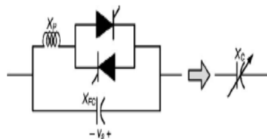
Fig 2 Equivalent circuit of TCSC
